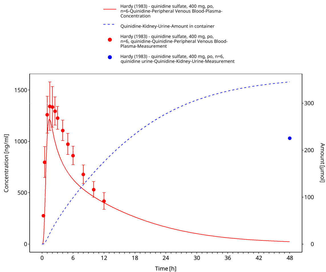
Figure 3-33: Hardy 1983: quinidine sulfate, 400 mg, po, n=6
