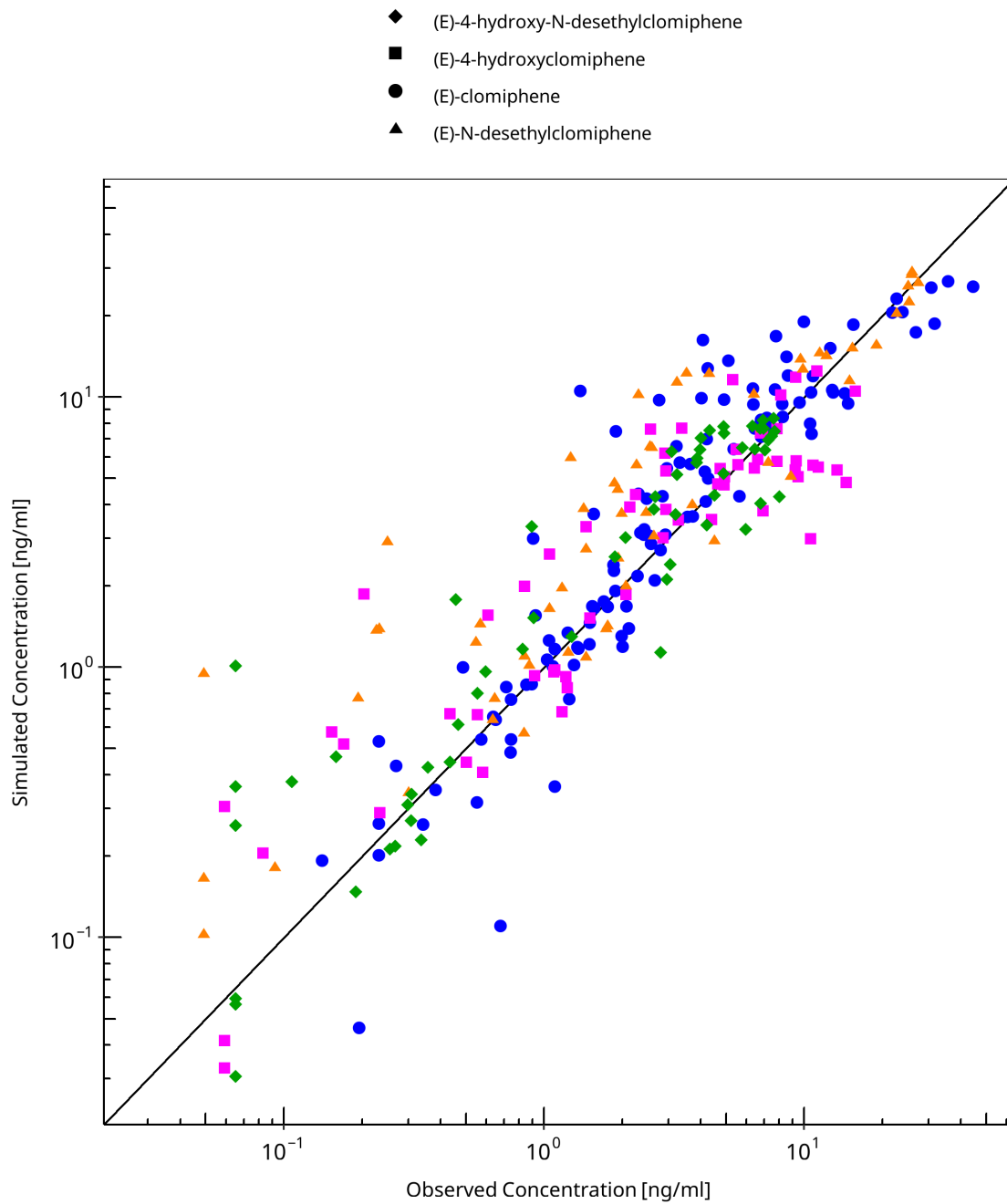
Figure 3-1: Observed versus simulated concentration-time data for all modeled compounds
