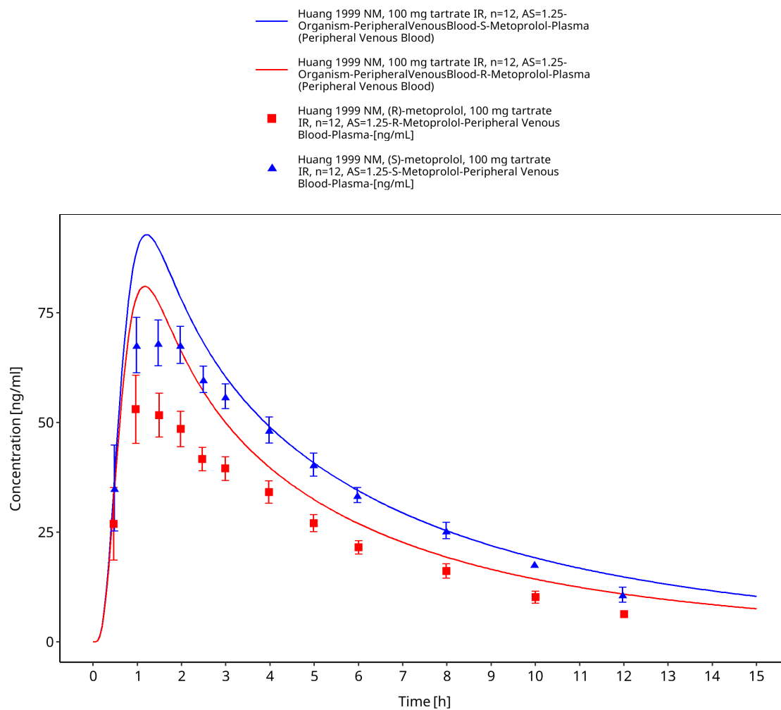
Figure 3-11: Huang 1999: NM, 100 mg tartrate IR, n=12, AS=1.25
