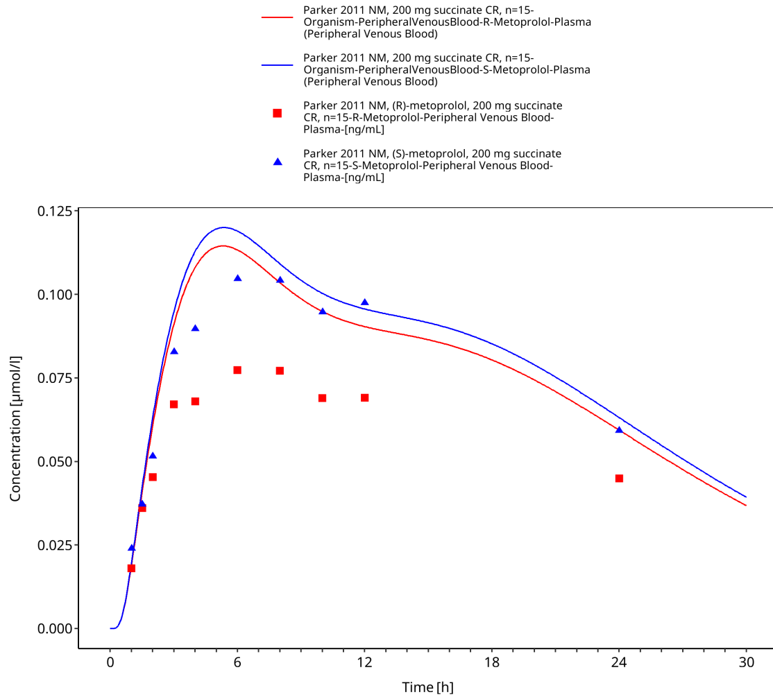
Figure 3-44: Parker 2011: NM, 200 mg succinate CR, n=15
