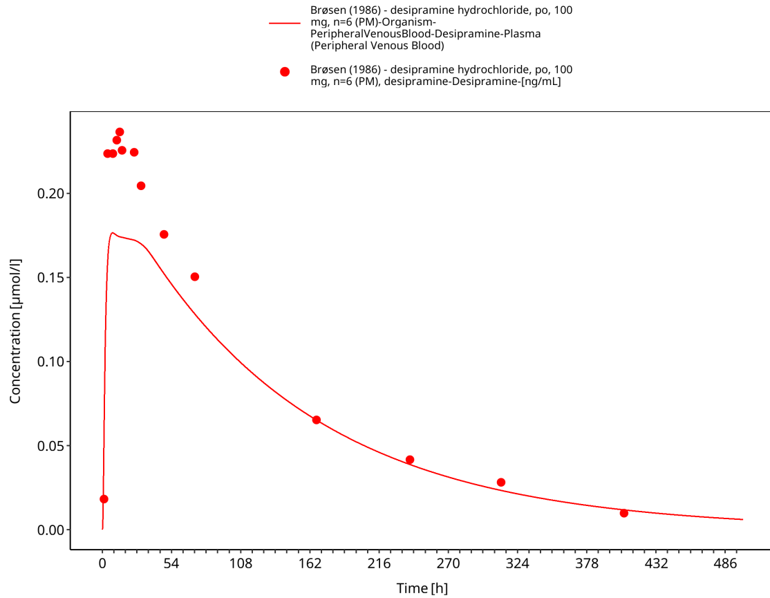
Figure 3-8: Brøsen 1986: desipramine hydrochloride, po, 100 mg, n=6 (PM)
