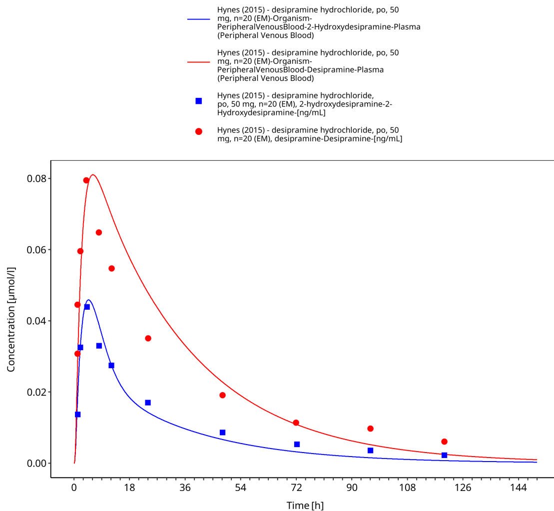
Figure 3-20: Hynes 2015: desipramine hydrochloride, po, 50 mg, n=20 (EM)
