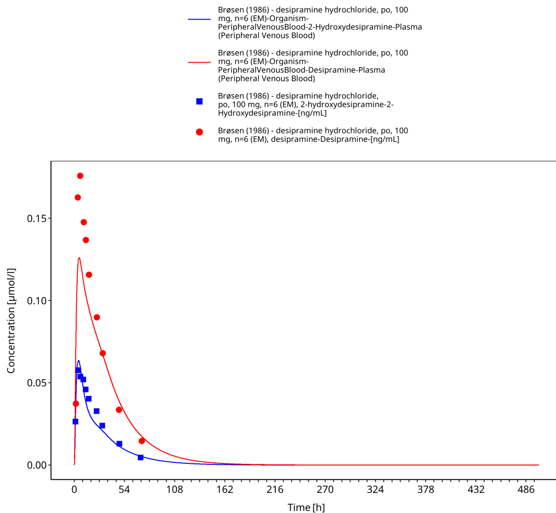
Figure 3-9: Brøsen 1986: desipramine hydrochloride, po, 100 mg, n=6 (EM)
