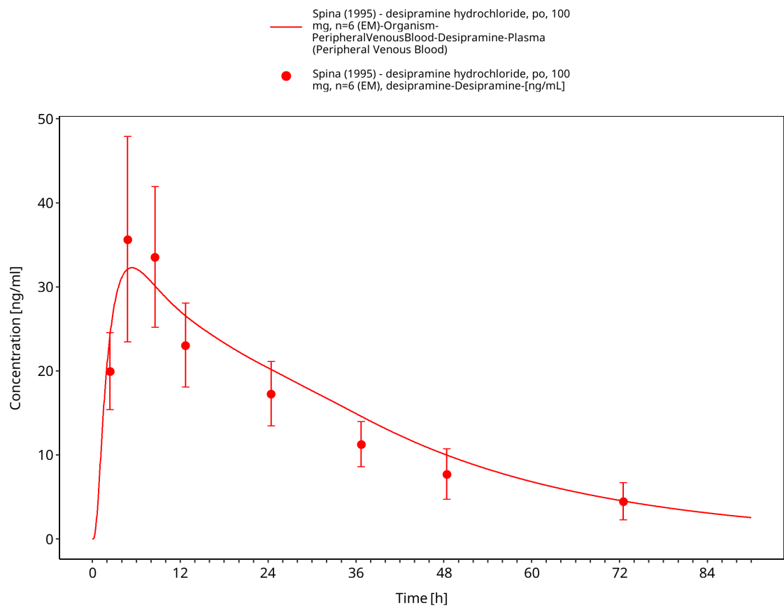
Figure 3-24: Spina 1995: desipramine hydrochloride, po, 100 mg, n=6 (EM)
