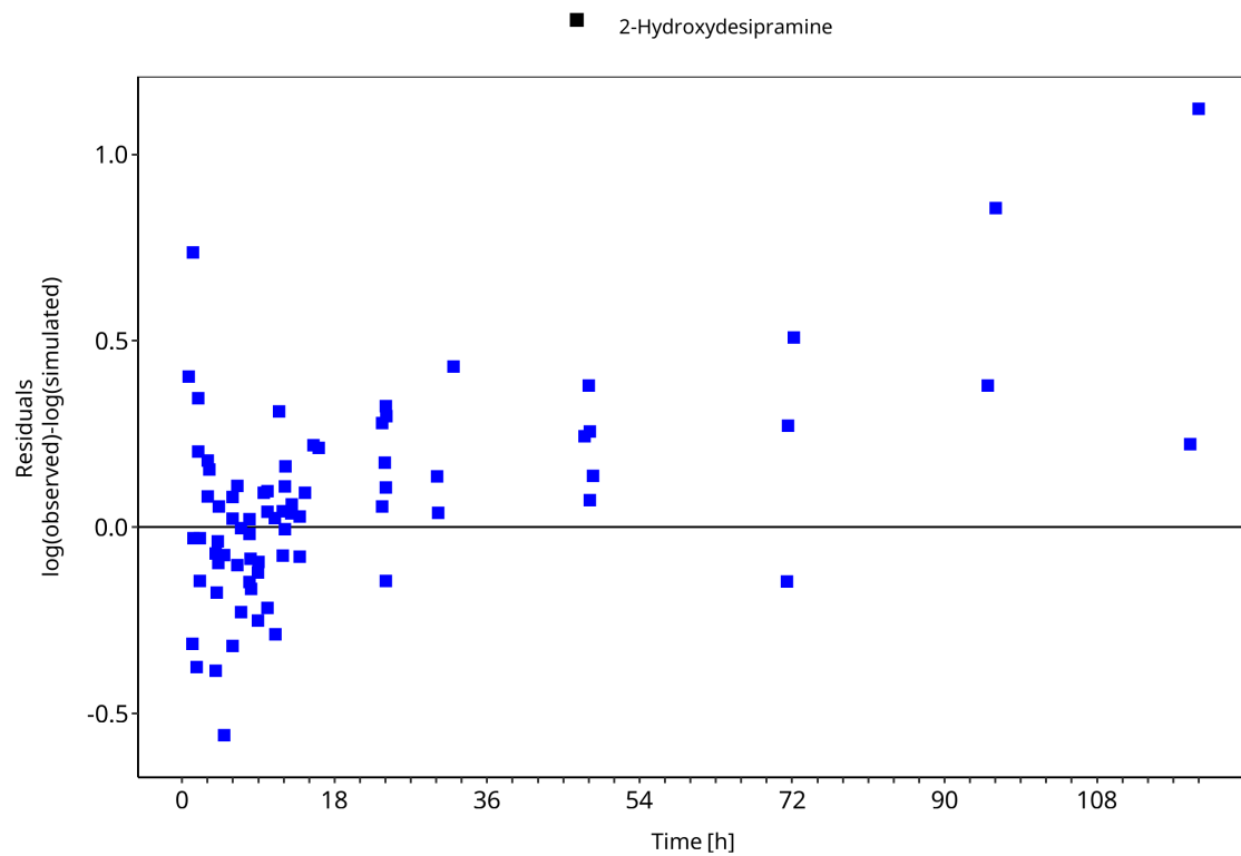
Figure 3-4: 2-Hydroxydesipramine goodness-of-fit diagnostics
