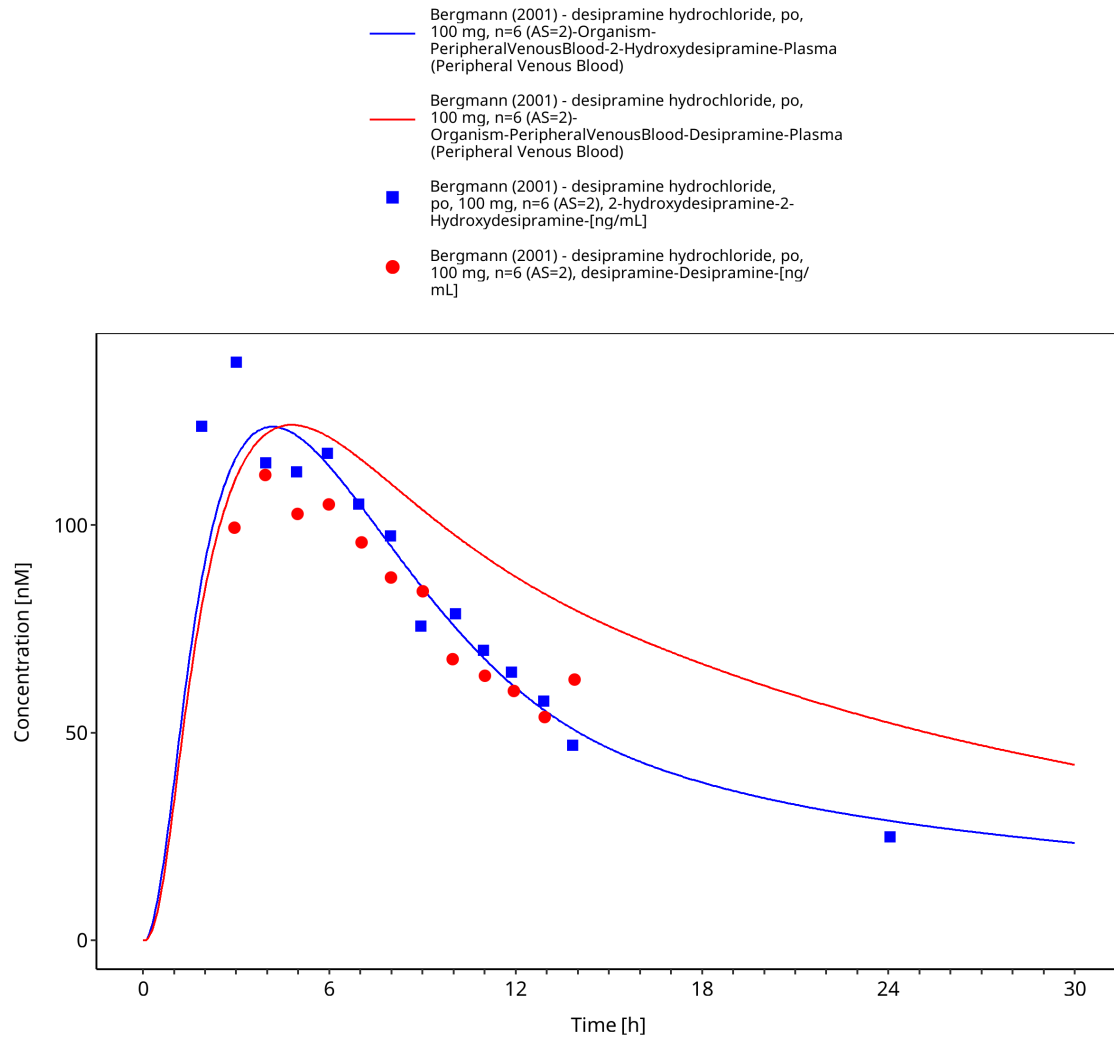
Figure 3-17: Bergmann 2001: desipramine hydrochloride, po, 100 mg, n=6 (AS=2)
