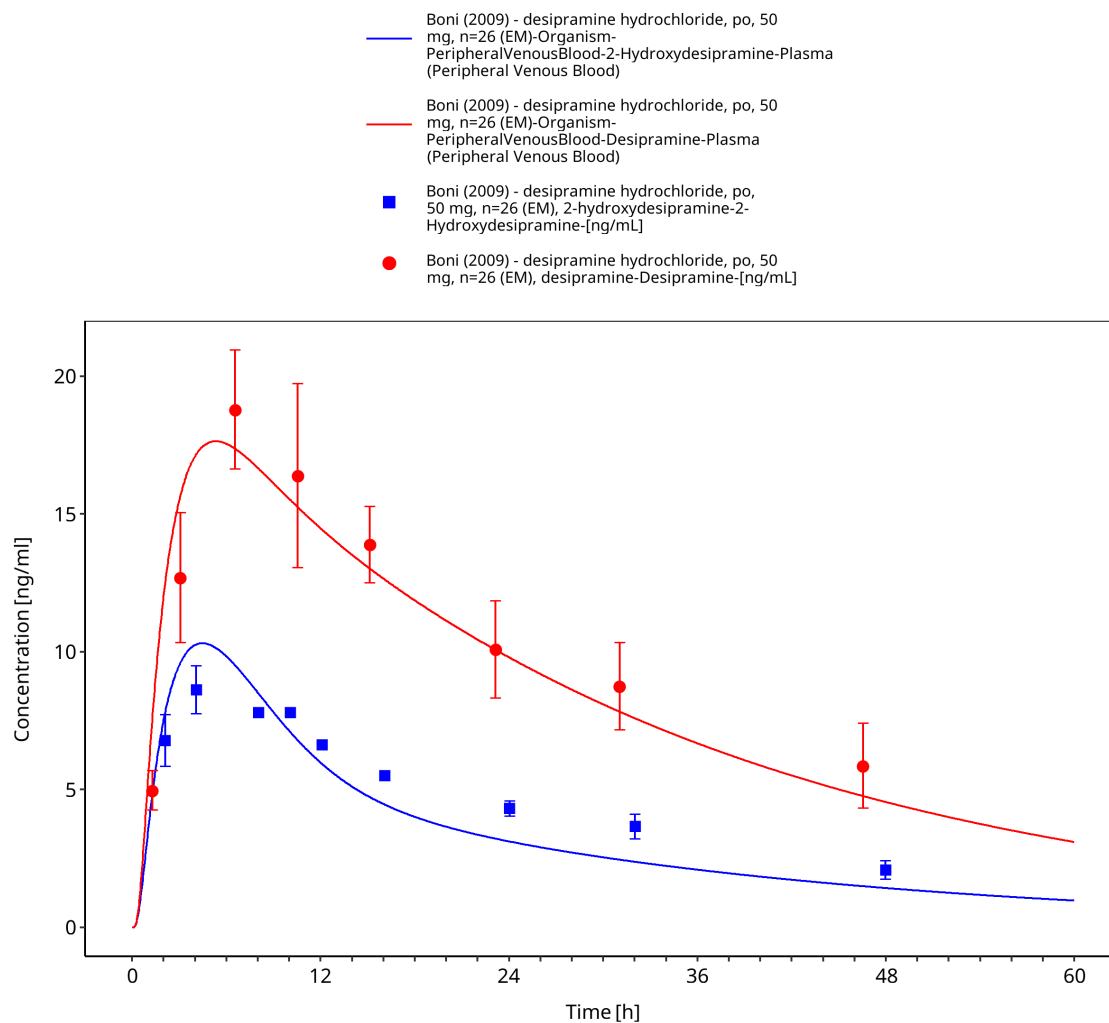
Figure 3-6: Boni 2009: desipramine hydrochloride, po, 50 mg, n=26 (EM)
