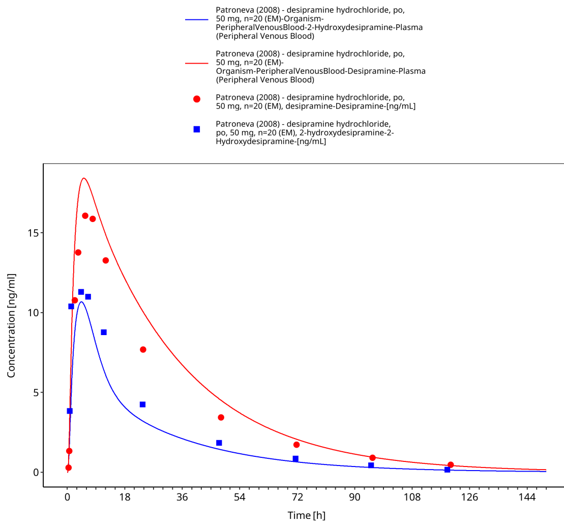
Figure 3-22: Patroneva 2008: desipramine hydrochloride, po, 50 mg, n=20 (EM)
