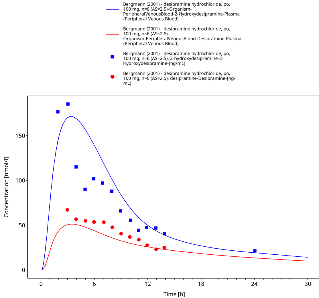
Figure 3-18: Bergmann 2001: desipramine hydrochloride, po, 100 mg, n=6 (AS=2.5)
