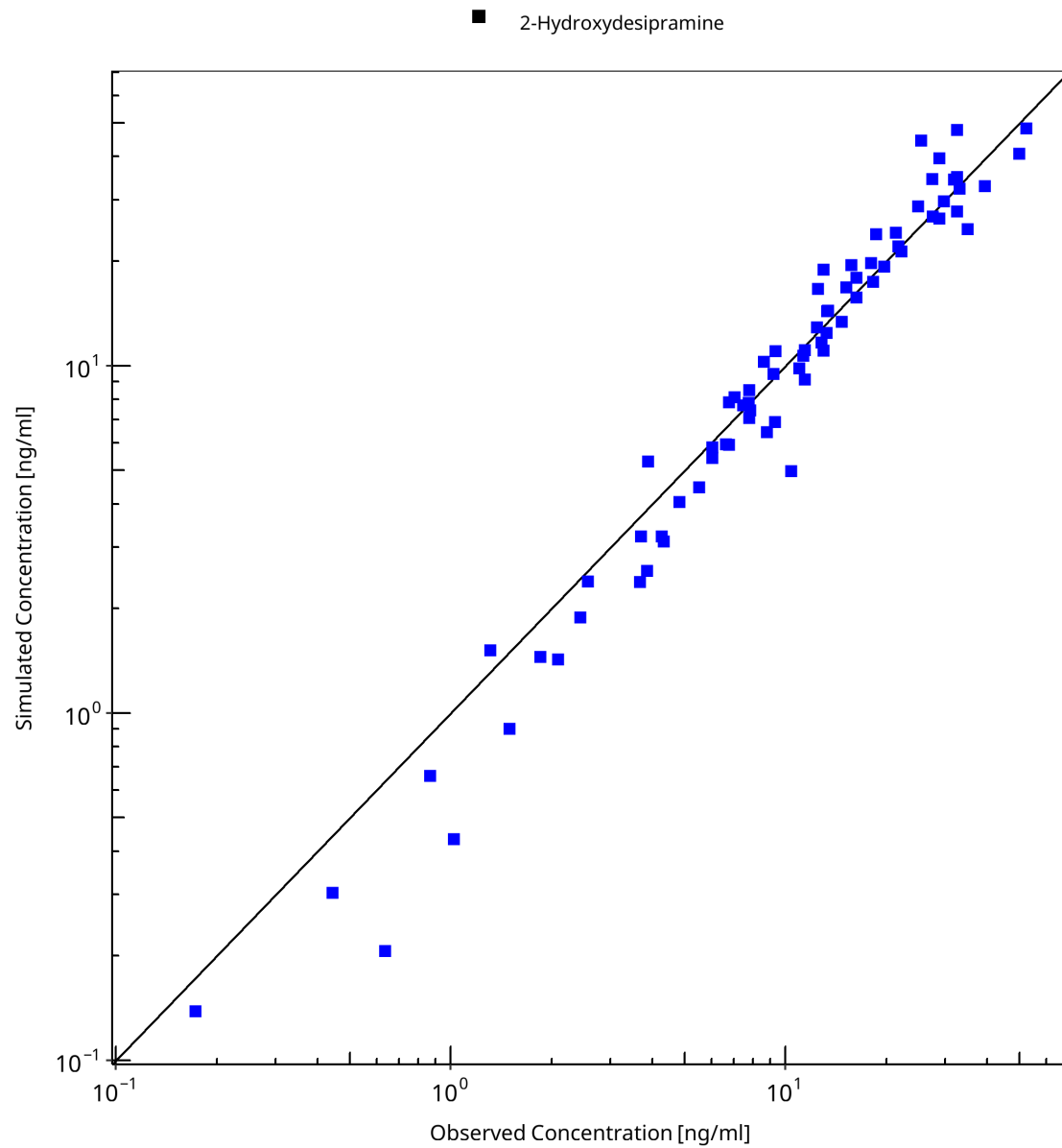
Figure 3-3: 2-Hydroxydesipramine goodness-of-fit diagnostics
