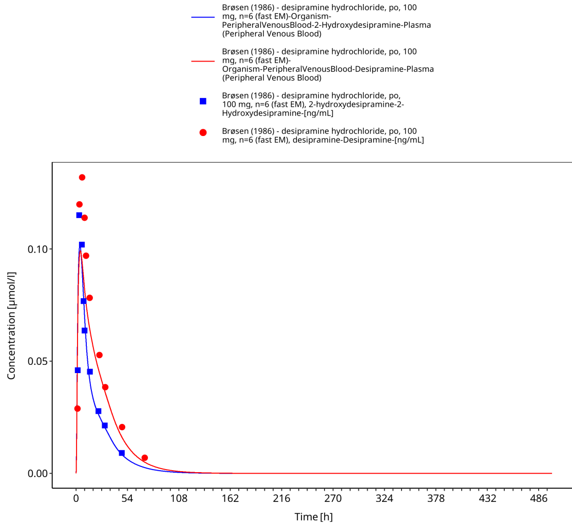
Figure 3-7: Brøsen 1986: desipramine hydrochloride, po, 100 mg, n=6 (fast EM)
