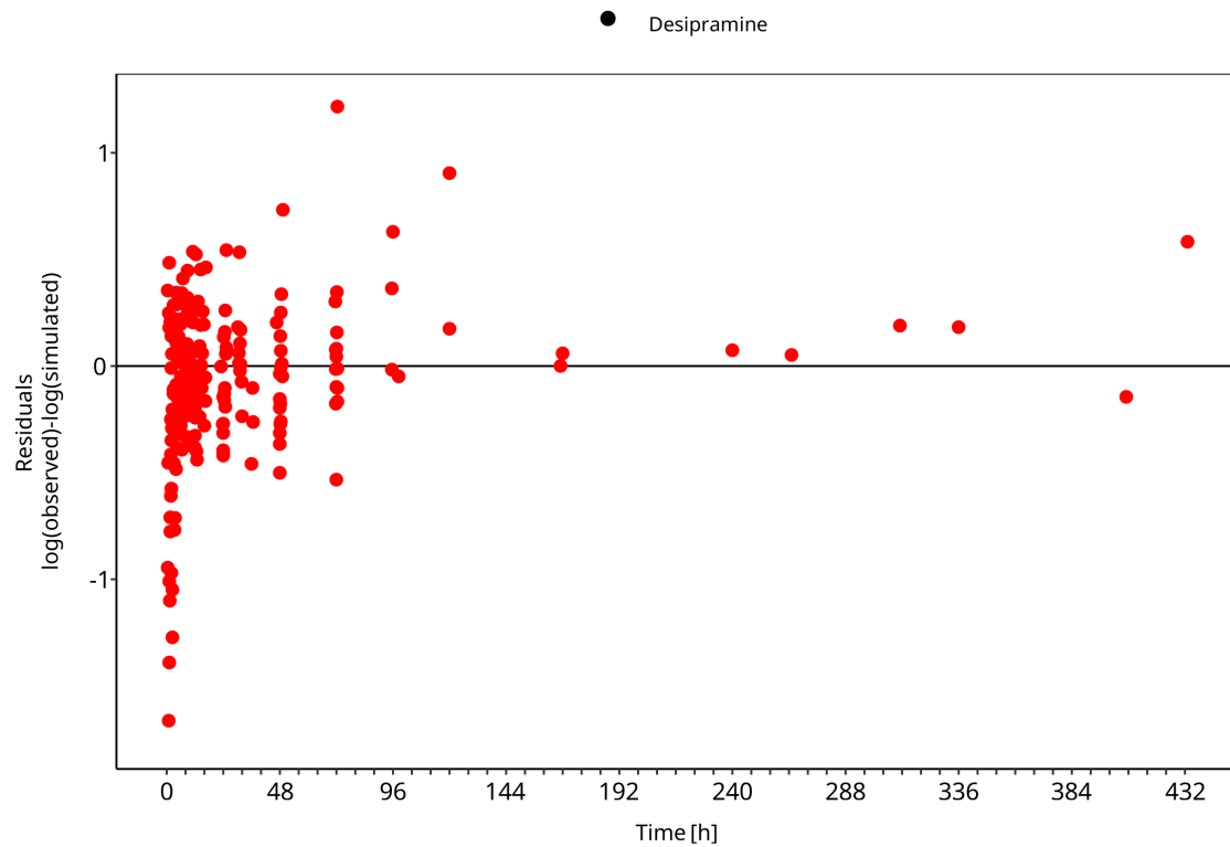
Figure 3-2: Desipramine goodness-of-fit diagnostics
