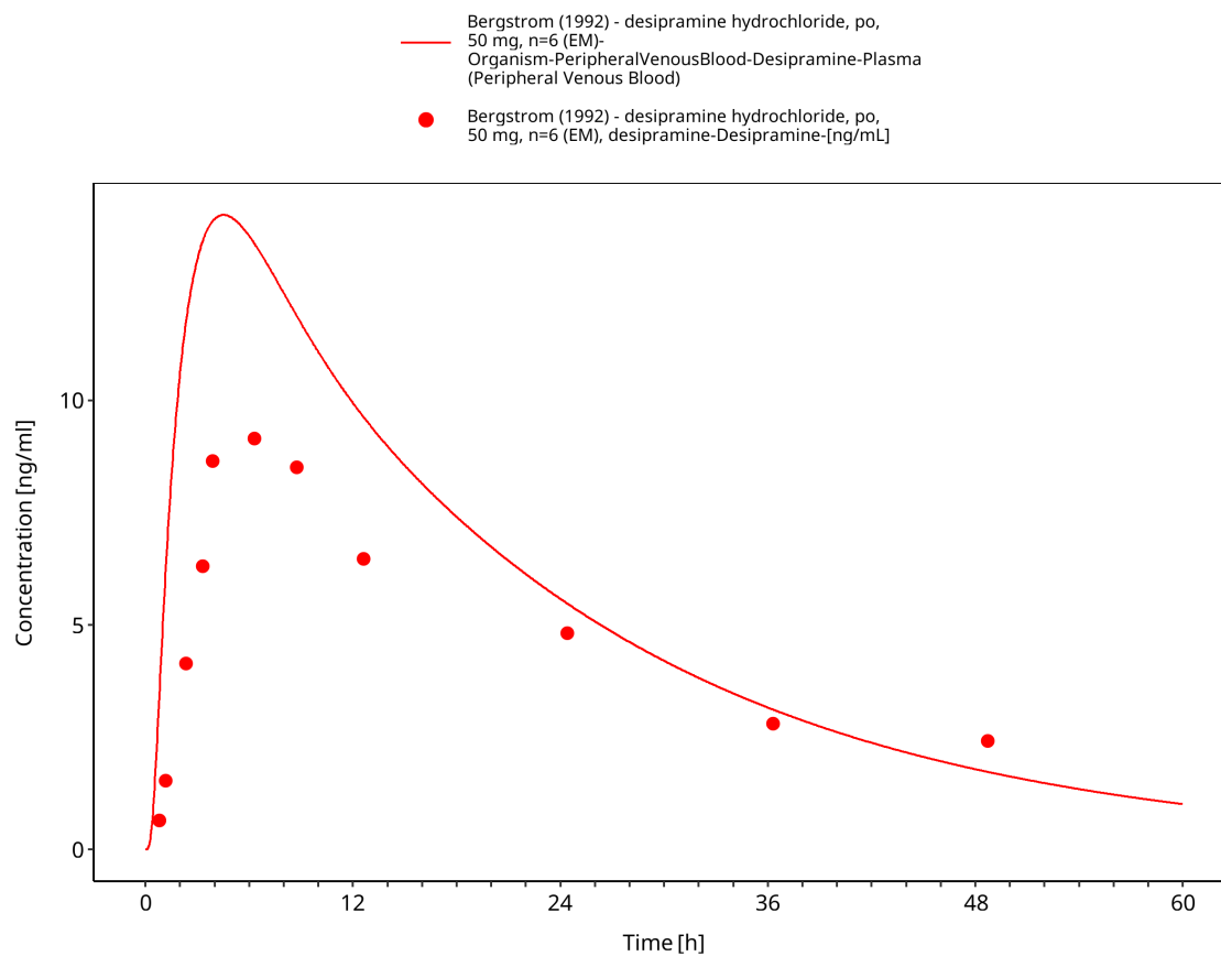
Figure 3-19: Bergstrom 1992: desipramine hydrochloride, po, 50 mg, n=6
