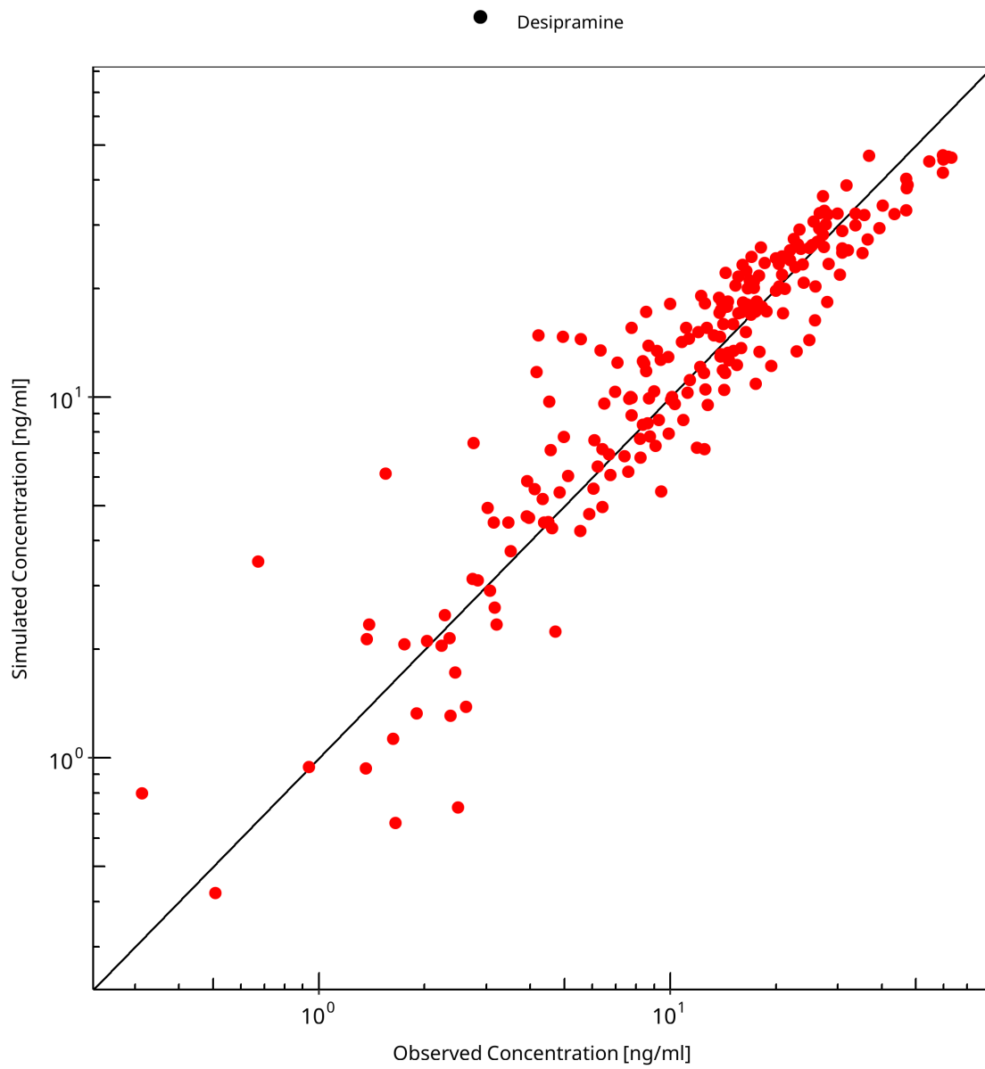
Figure 3-1: Desipramine goodness-of-fit diagnostics
