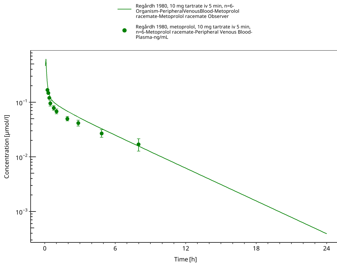
Figure 3-45: Regårdh 1980: 10 mg tartrate iv 5 min, n=6
