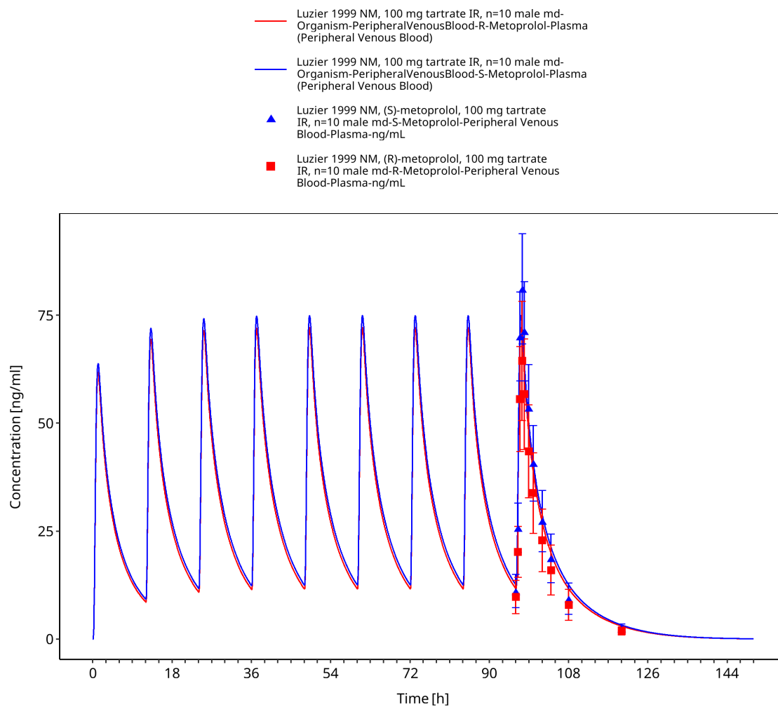
Figure 3-41: Luzier 1999: NM, 100 mg b.i.d. tartrate IR, n=10 male, multiple dose
