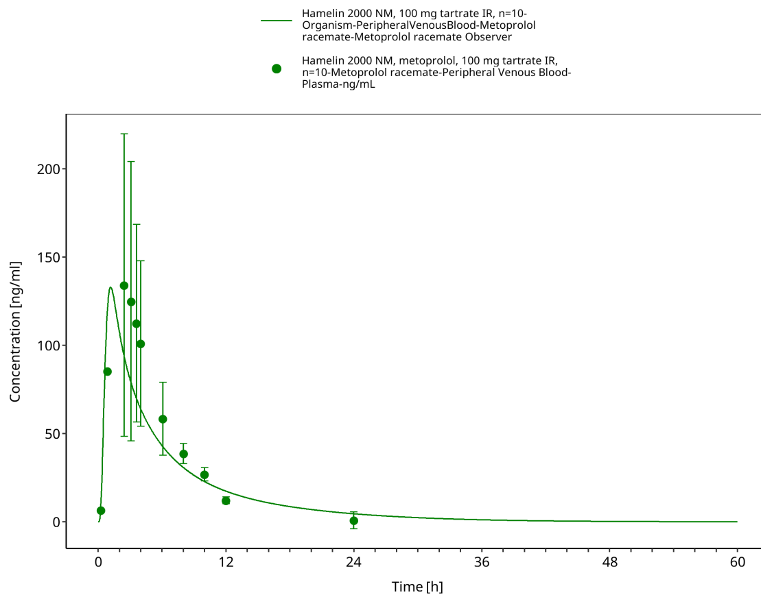
Figure 3-30: Hamelin 2000: NM, 100 mg tartrate IR, n=10
