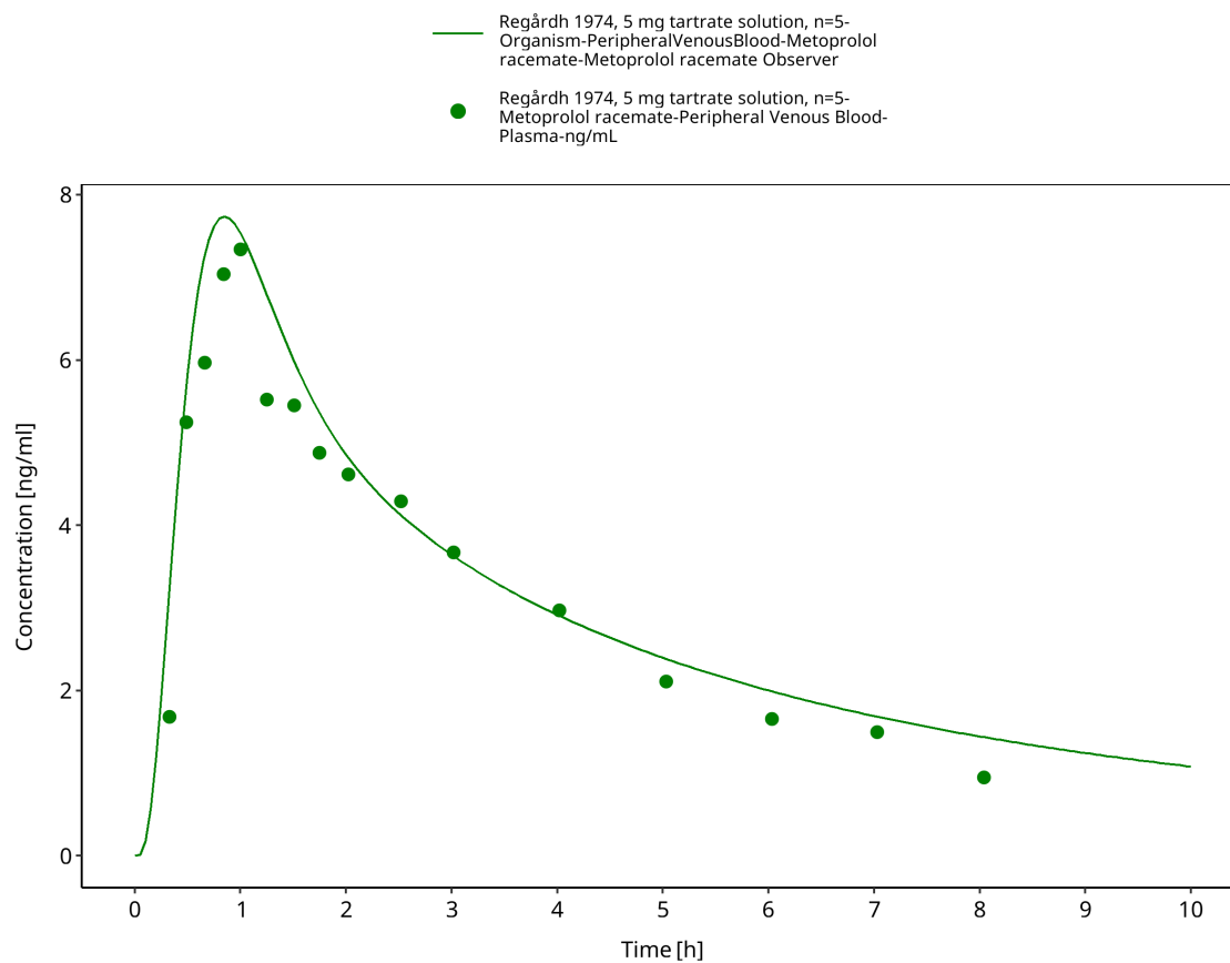
Figure 3-24: Regårdh 1974: 5 mg tartrate solution, n=5
