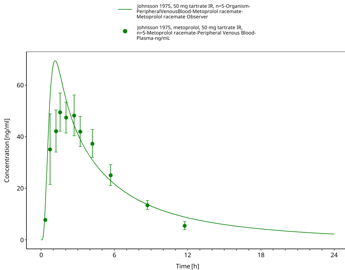
Figure 3-37: Johnsson 1975: 50 mg tartrate IR, n=5
