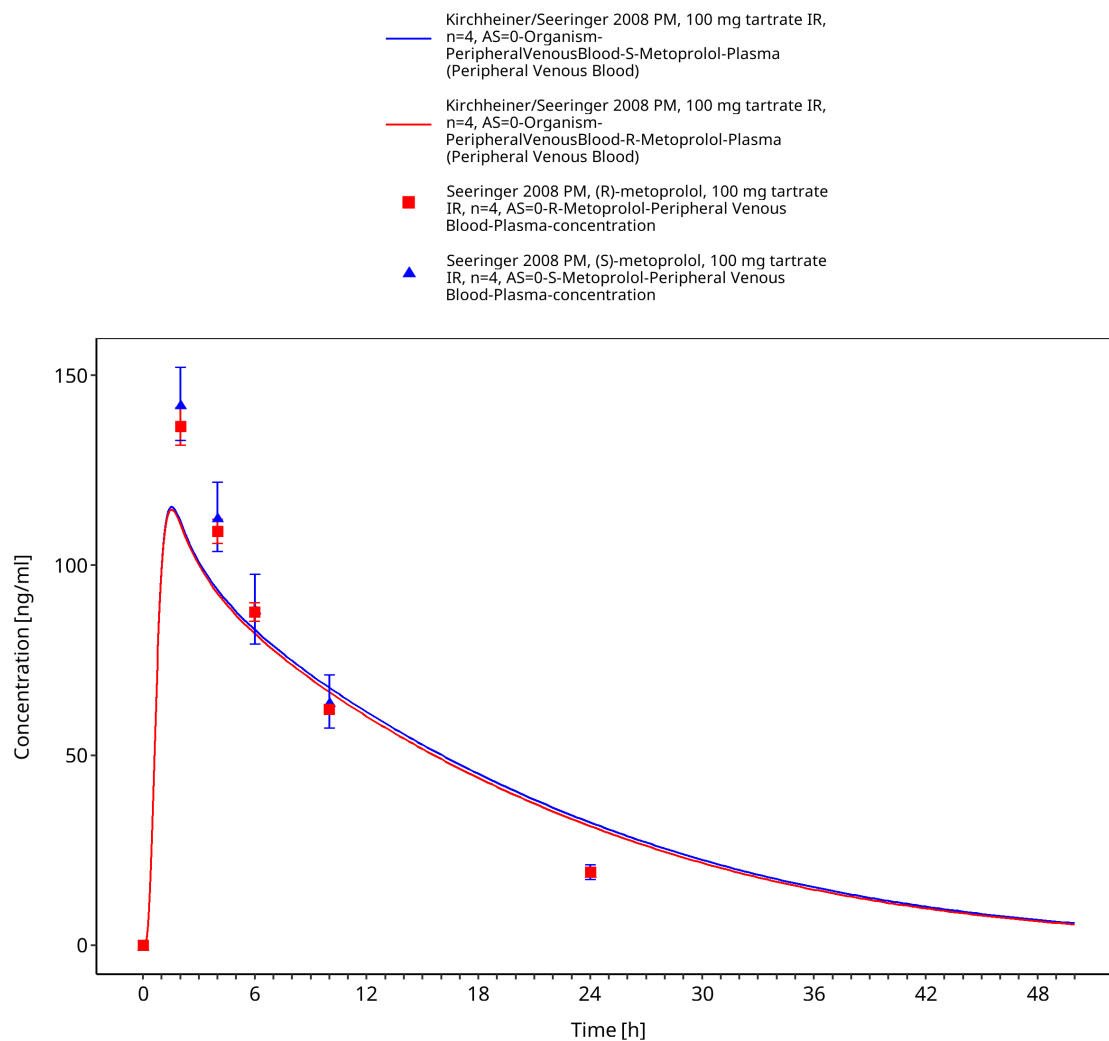
Figure 3-21: Kirchheiner 2004 / Seeringer 2008: PM, 100 mg tartrate IR, n=4, AS=0
