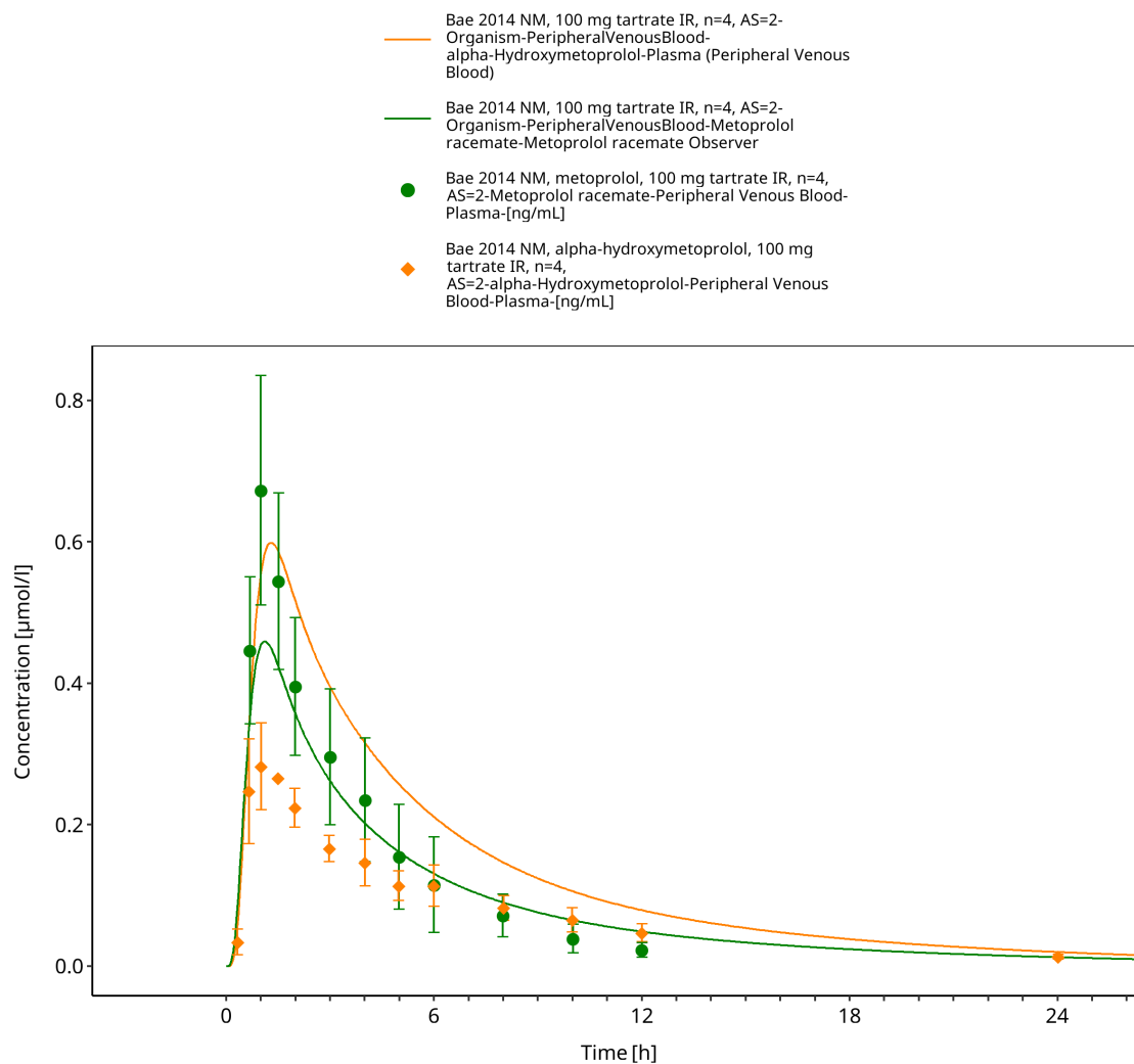
Figure 3-28: Bae 2014: NM, 100 mg tartrate IR, n=4, AS=2
