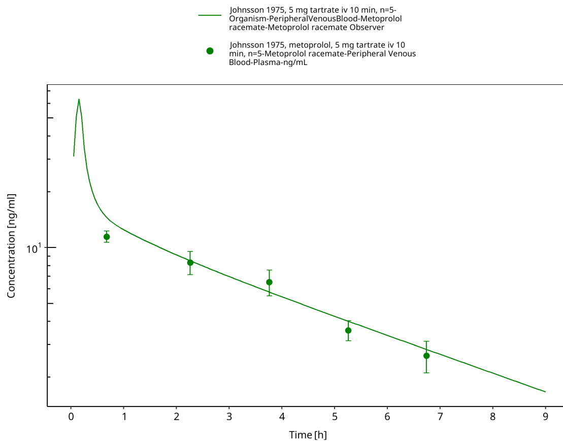
Figure 3-32: Johnsson 1975: 5 mg tartrate iv 10 min, n=5
