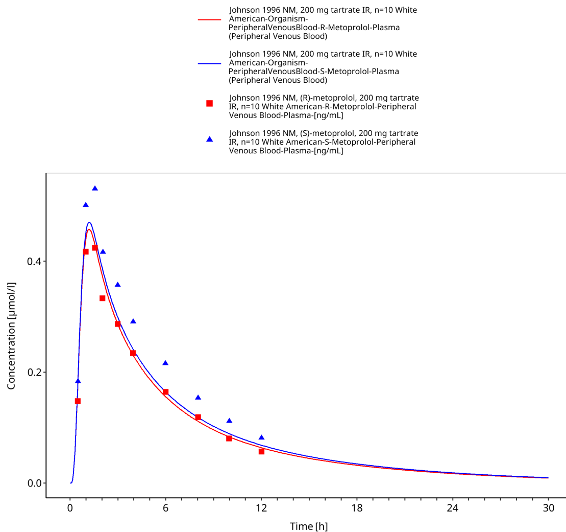
Figure 3-17: Johnson 1996: NM, 200 mg tartrate IR, n=10 White American
