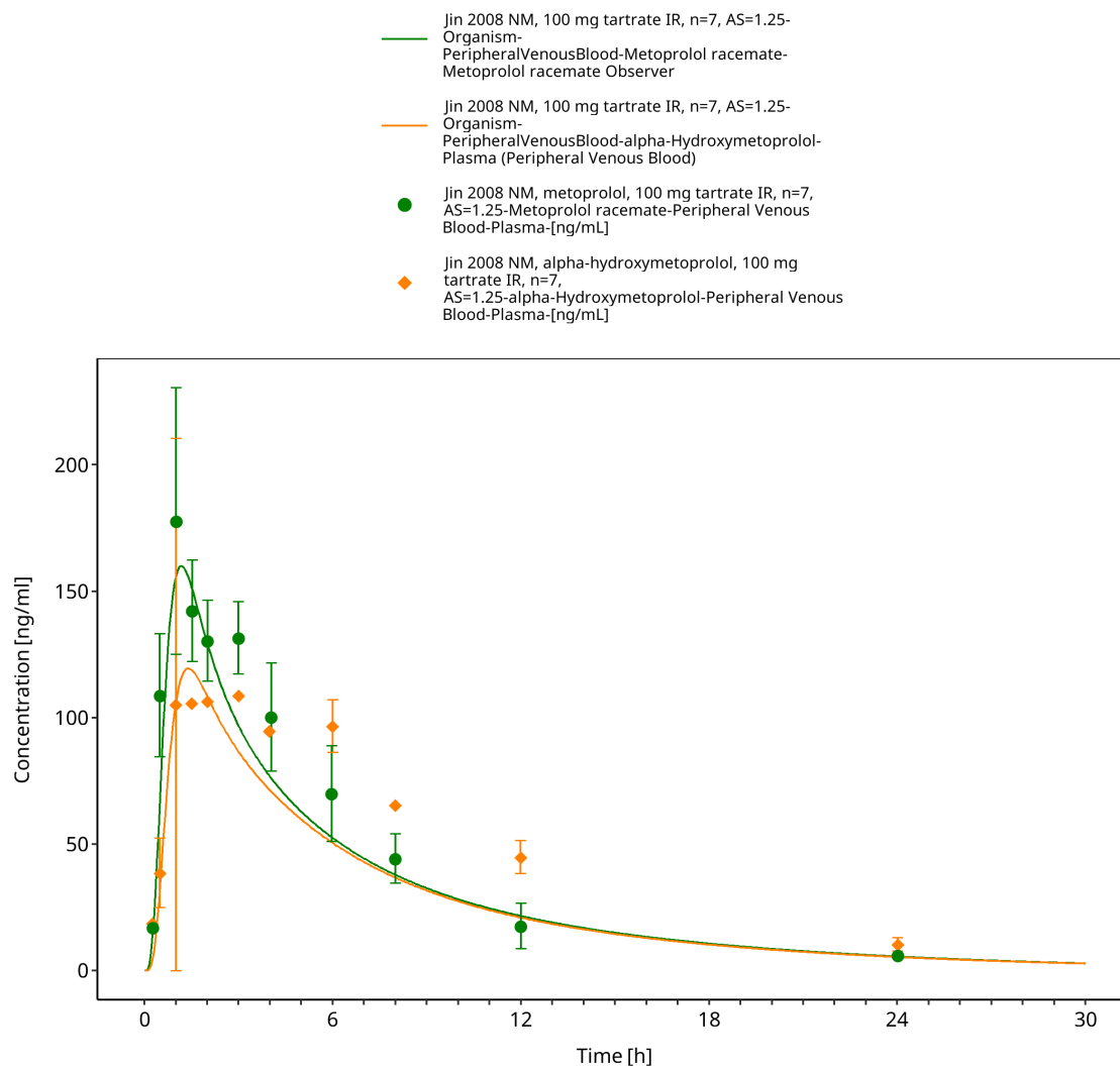
Figure 3-14: Jin 2008: NM, 100 mg tartrate IR, n=7, AS=1.25
