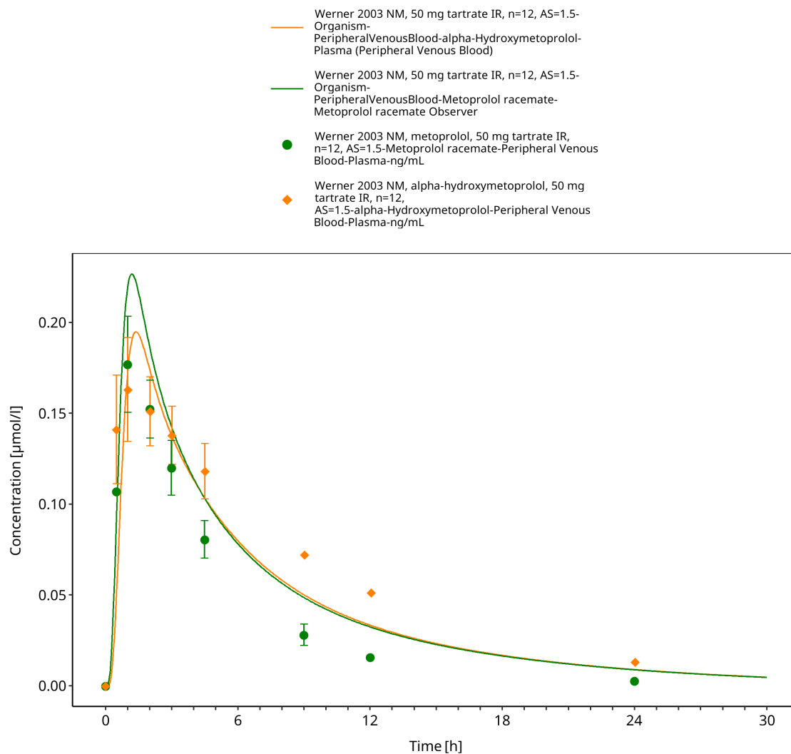
Figure 3-48: Werner 2003: NM, 50 mg tartrate IR, n=12, AS=1.5
