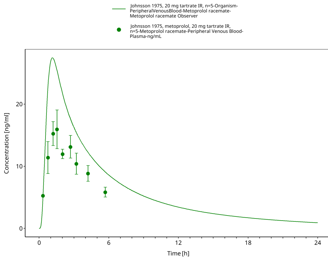
Figure 3-35: Johnsson 1975: 20 mg tartrate IR, n=5
