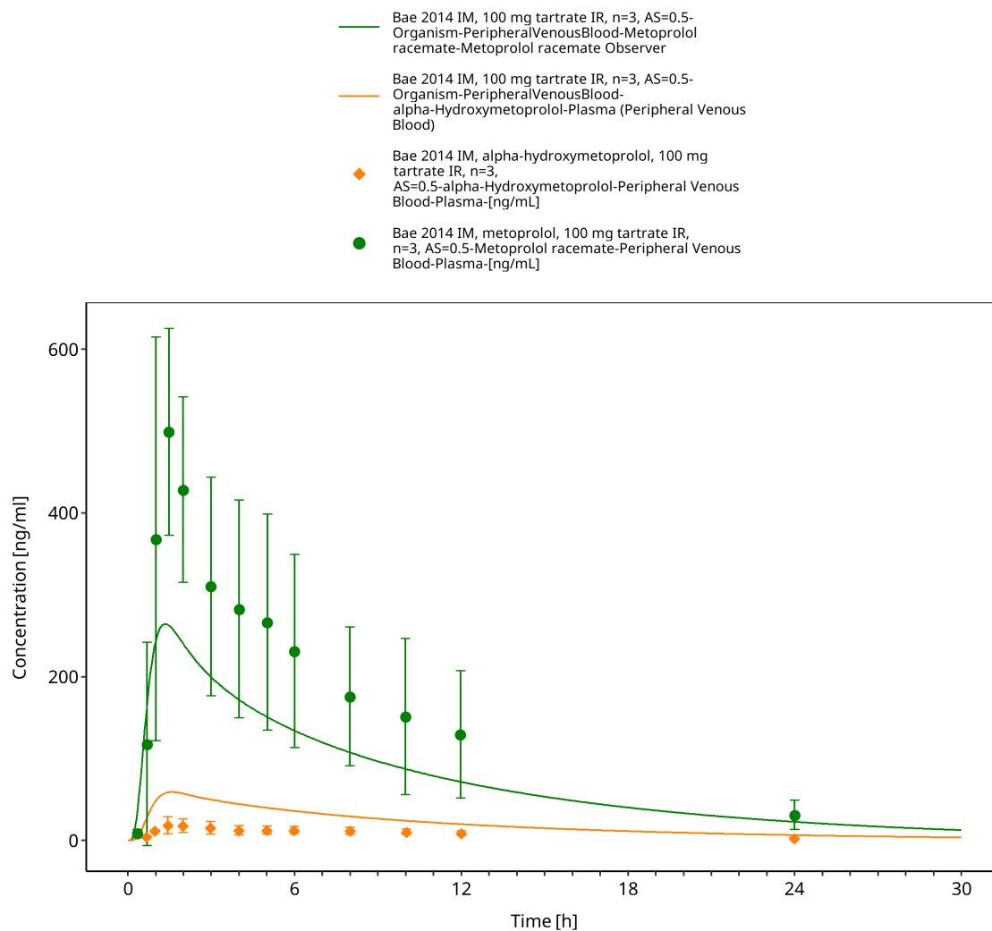
Figure 3-27: Bae 2014: IM, 100 mg tartrate IR, n=3, AS=0.5
