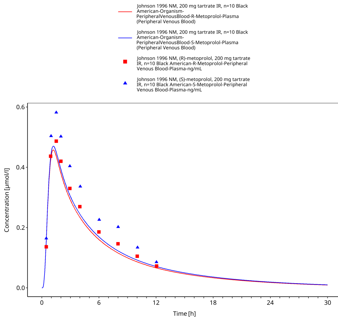
Figure 3-16: Johnson 1996: NM, 200 mg tartrate IR, n=10 Black American
