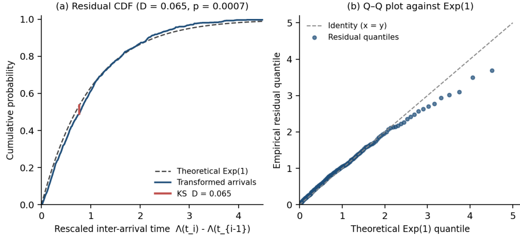
Figure 5.18: Self-excitation in the handover arrival stream. While the Ogata residual test formally rejects the stationary exponential kernel ( D = 0.065 , p = 0.0007 , likely due to time-varying background rate and corridor transitions), the fitted intensity captures the strong empirical clustering of handovers into bursts.
