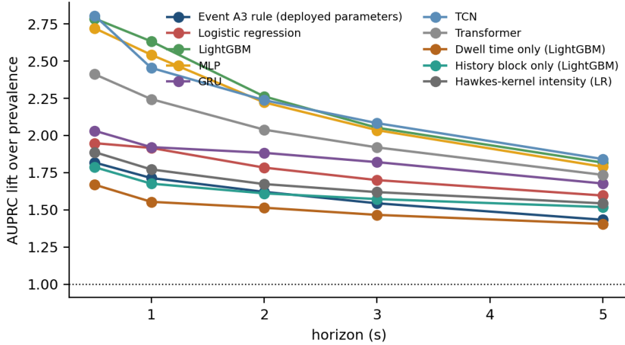
Figure 5.3: AUPRC lift over the prevalence floor by horizon across learners, out of fold under leave-one-campaign-out. LightGBM, MLP, and TCN achieve comparable performance within overlapping bootstrap intervals (pooled 1 s AUPRC 0.179, 0.173, and 0.167 respectively), all significantly exceeding the prevalence floor and the A3 signal-margin proxy.
