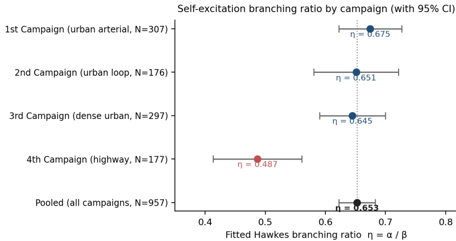
Figure 5.17: Hawkes branching ratio estimated on each campaign separately and on the pooled stream, with bootstrap confidence intervals. While sub-critical branching ratios indicate substantial empirical clustering ( \hat{\eta} \approx 0.49\text{--}0.68 ), the stationary exponential-kernel model is rejected by Ogata residual testing ( p = 0.0007 ), so the ratio is reported as an index of clustering rather than a validated structural generative model.
