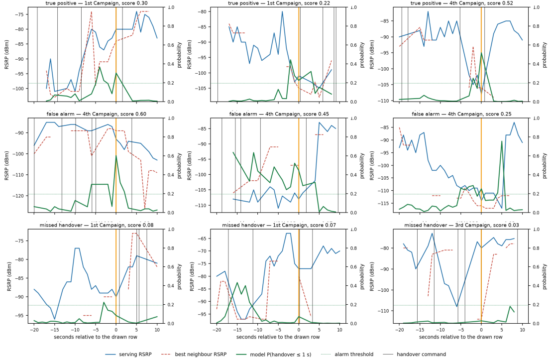
Figure 5.20: Nine cases drawn uniformly at random, with a fixed seed, from the out-of-fold predictions at the 5 % false-positive operating point. Blue: serving RSRP (1 Hz export); Red: best neighbour RSRP (zero-order hold from decoded reports, with median observation age \approx 0.27 s); Green: model probability of command within 1 s. Traces reflect observed feature patterns rather than continuous internal PHY/RRC state machines.
