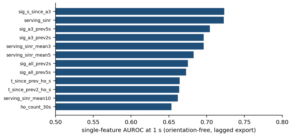
Figure 5.12: Single-feature discriminative power at one second on the lagged export. No single feature reaches the multivariate model.
