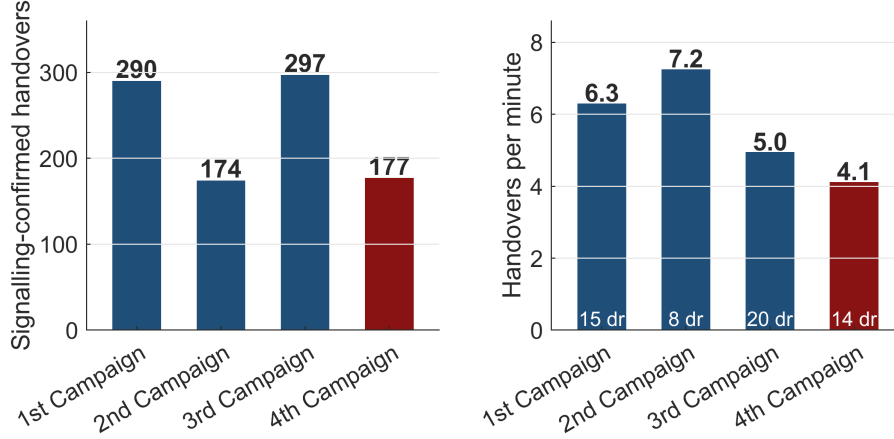
Figure 3.4: Composition of the pooled dataset across the four campaigns. In the event panel, counts reflect the N = 938 handover commands falling within retained quality-controlled blocks (290, 174, 297, and 177 respectively), which feed the feature pipeline, drawn from the 957 total decoded commands in Table 3.2.
