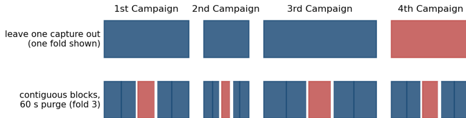
Figure 4.2: The splitting ladder. Leave-one-campaign-out holds out a whole continuous session; blocked splitting holds out time blocks; random-row splitting holds out individual samples, allowing near-duplicate rows across splits.
