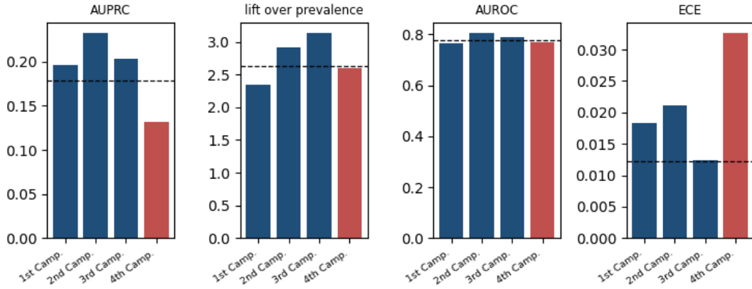
Figure 5.10: Leave-one-campaign-out on four metrics. Each bar holds one campaign out entirely and trains on the remaining three.
