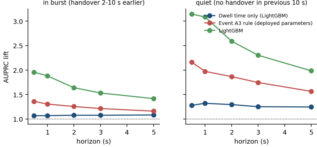
Figure 5.8: Where the model earns its advantage: rows with no handover in the previous ten seconds against rows within a burst. The model predicts both isolated and burst arrivals effectively.
