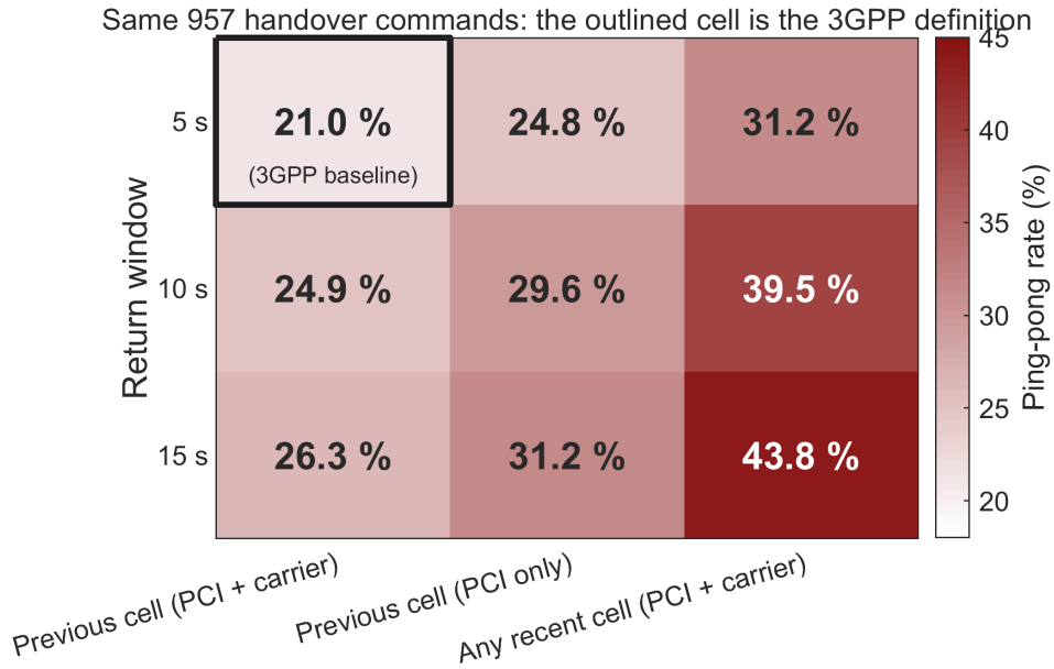
Figure 5.15: The ping-pong rate over the full definitional grid: three return windows against three conventions for cell identity and return, computed on one unchanging set of 957 handover commands.
