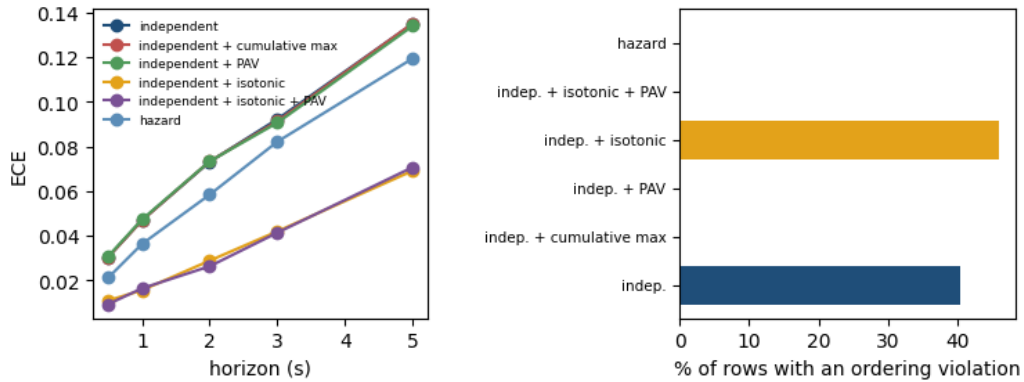
Figure 5.7: Calibration error against the horizon for every coherence arm (left) and the share of rows with coherence violations (right). The hazard formulation achieves zero violations.
