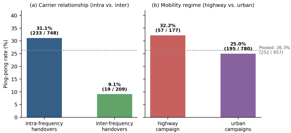
Figure 5.16: Where ping-pong concentrates. The dominant axis is the carrier relationship, not the mobility regime.
