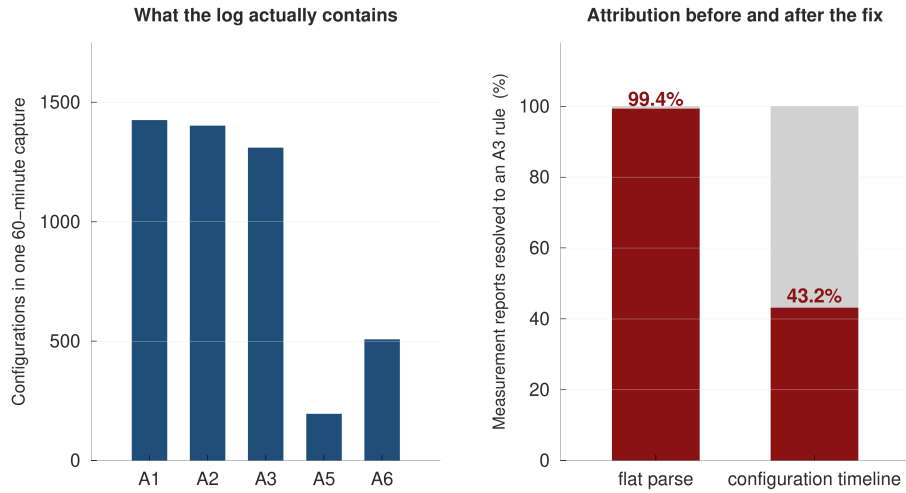
Figure 3.2: Measurement identifiers persist in VarMeasConfig until they are modified or removed. A flat union of report configurations overstates the active set; the timeline resolves each report against the configuration in force at its own timestamp.
