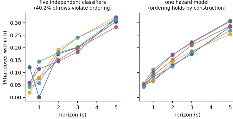
Figure 4.1: Independent per-horizon classifiers against the hazard formulation, drawn on simulated rows. The hazard formulation enforces monotonicity across horizons by construction.
