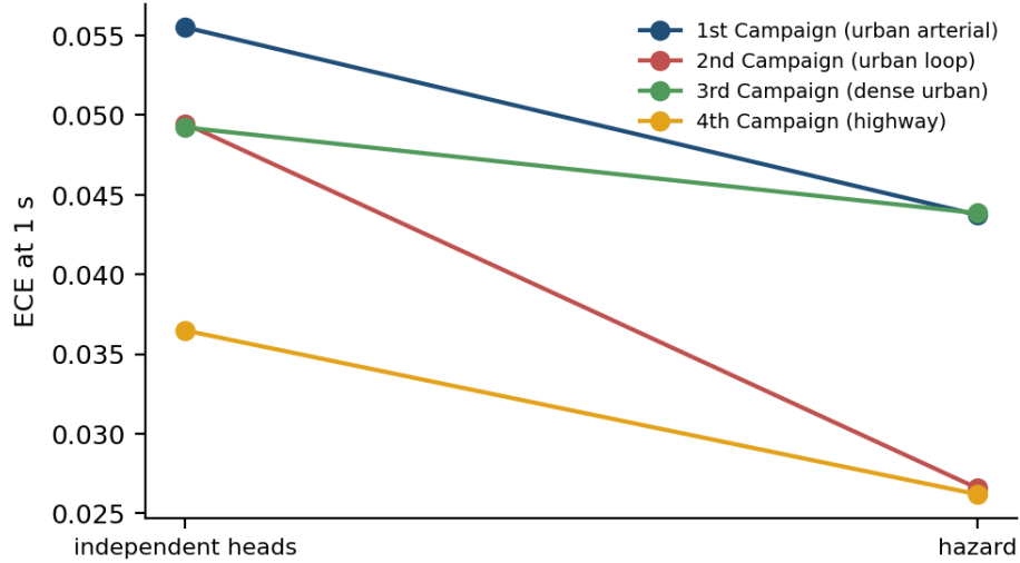
Figure 5.6: Calibration error at one second, one line per held-out campaign, for independent classifiers against the hazard formulation. The hazard formulation reduces ECE across all folds.
