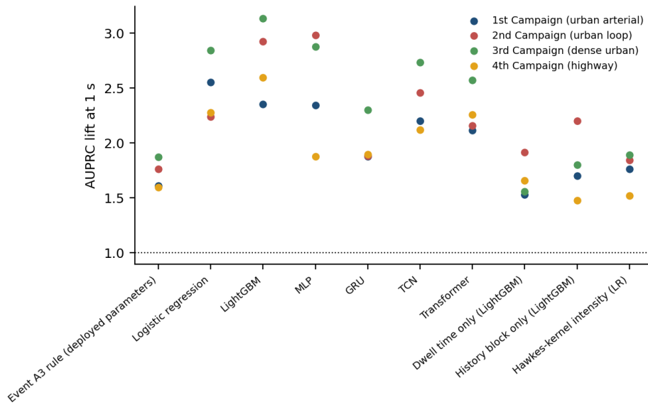
Figure 5.4: One-second AUPRC lift by learner, with each held-out campaign drawn separately. The spread reflects genuine inter-campaign variability in route and speed.
