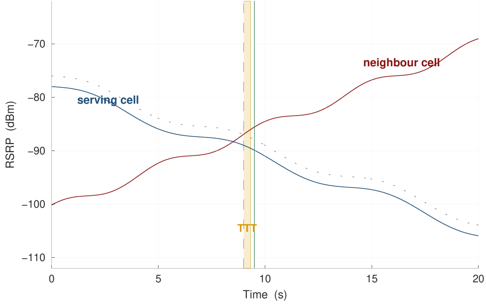
Figure 1.1: Event A3 fires only after the neighbour has been better than the serving cell by a configured offset for a configured time-to-trigger. The entry condition is strictly retrospective.
