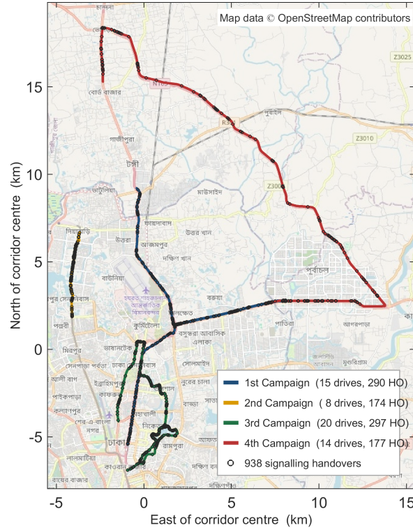
Figure 3.1: The four measurement campaigns on an OpenStreetMap background, including the central Dhaka urban corridors and the northern highway corridor up to Gazipur. Open circles mark signalling-confirmed handover commands ( N = 938 ).
