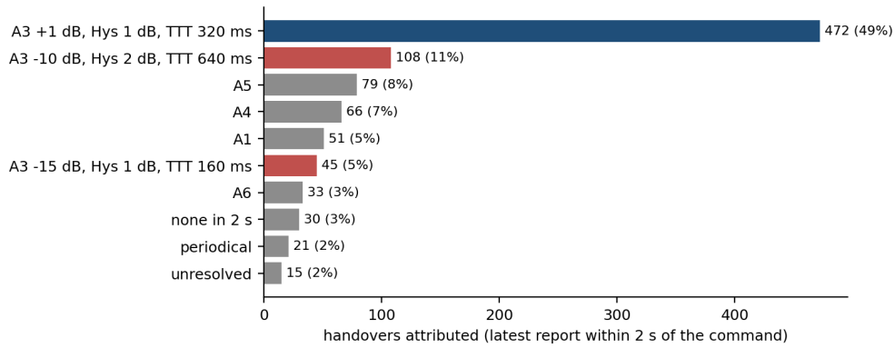
Figure 3.3: Handovers attributed to each configuration profile, weighted by the handovers each actually produced. Almost three quarters of all A3-triggered handovers occur under positive offsets, dominated by the +1 dB profile.
