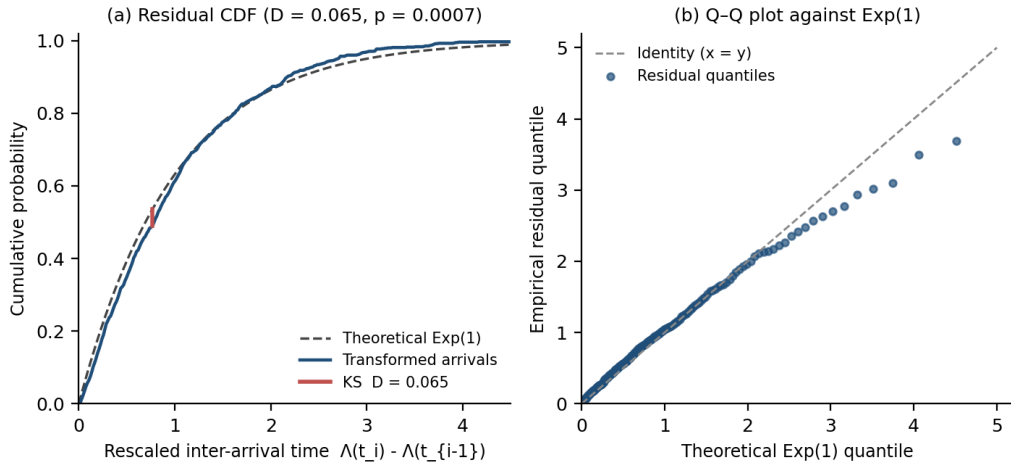
Figure 5.18: Self-excitation in the handover arrival stream. While the Ogata residual test formally rejects the stationary exponential kernel ( D = 0.065 , p = 0.0007 , likely due to time-varying background rate and corridor transitions), the fitted intensity captures the strong empirical clustering of handovers into bursts.
