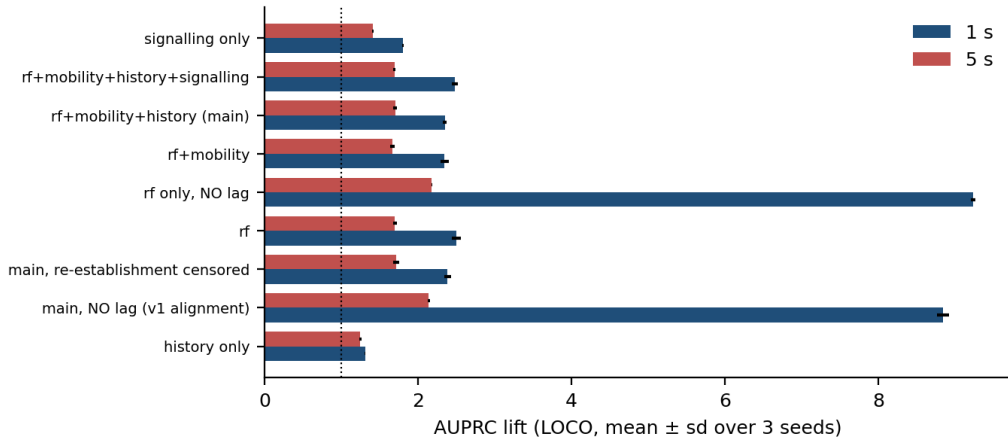
Figure 5.19: Feature-block, alignment and censoring ablations at one and five seconds, out of fold under leave-one-campaign-out.
