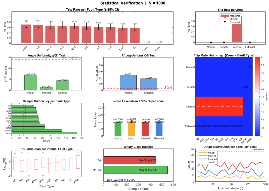
Figure 6.3: Statistical verification of the generated dataset.
