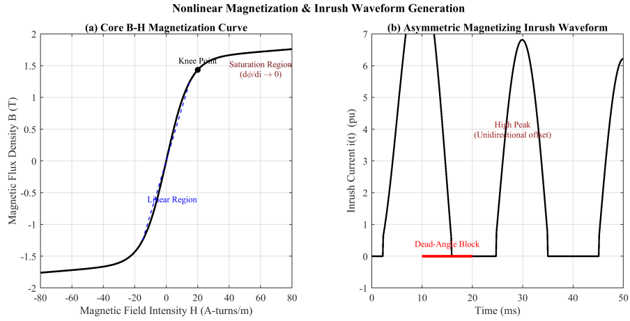
Figure 3.2: Core B-H saturation curve and the resulting magnetizing inrush waveform.
