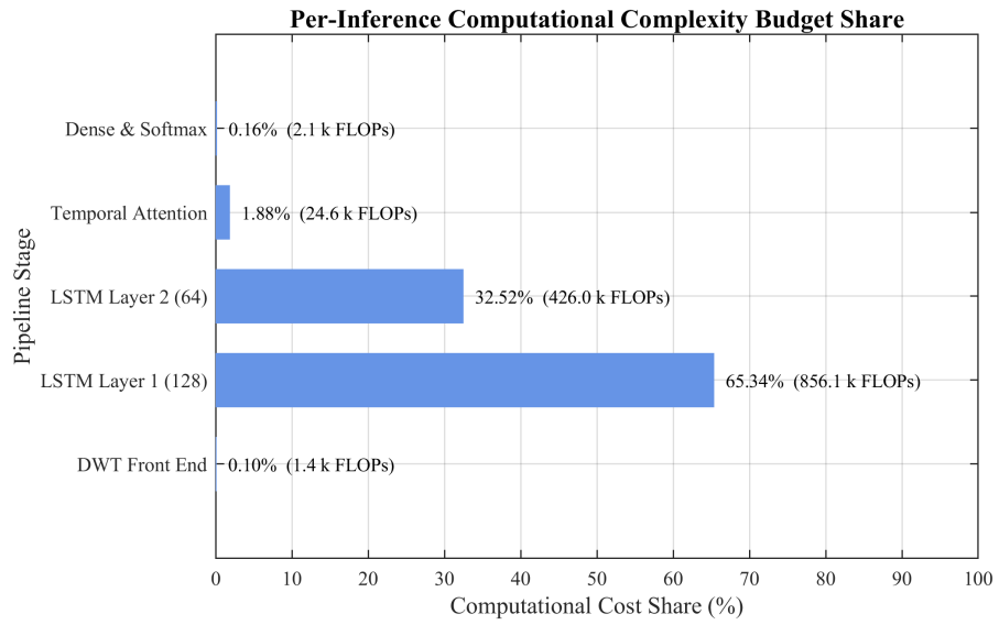
Figure 5.7: Per-inference computational cost distribution across pipeline stages.
