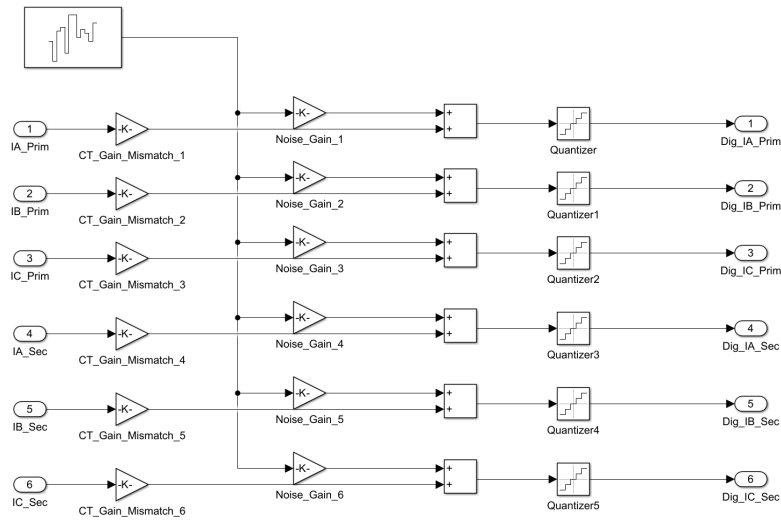
Figure 4.2: Block diagram of the merging-unit signal-conditioning and noise-injection pipeline.
