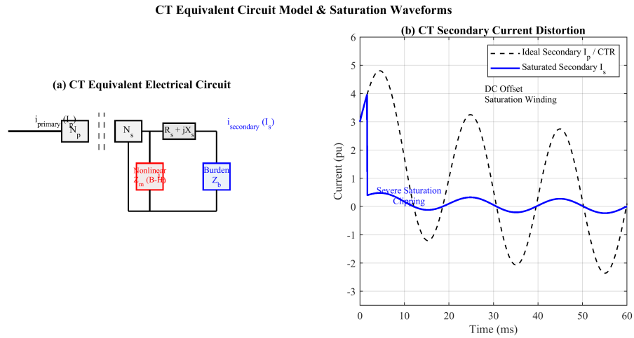
Figure 3.3: Current transformer equivalent circuit and saturation-induced secondary distortion.
