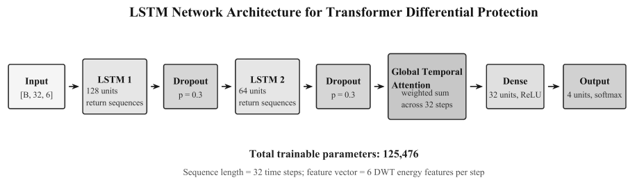
Figure 5.6: DWT-LSTM classifier architecture with global temporal attention.
