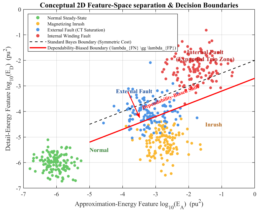
Figure 3.4: Conceptual feature-space separation of the four event classes with cost-asymmetric decision boundaries.
