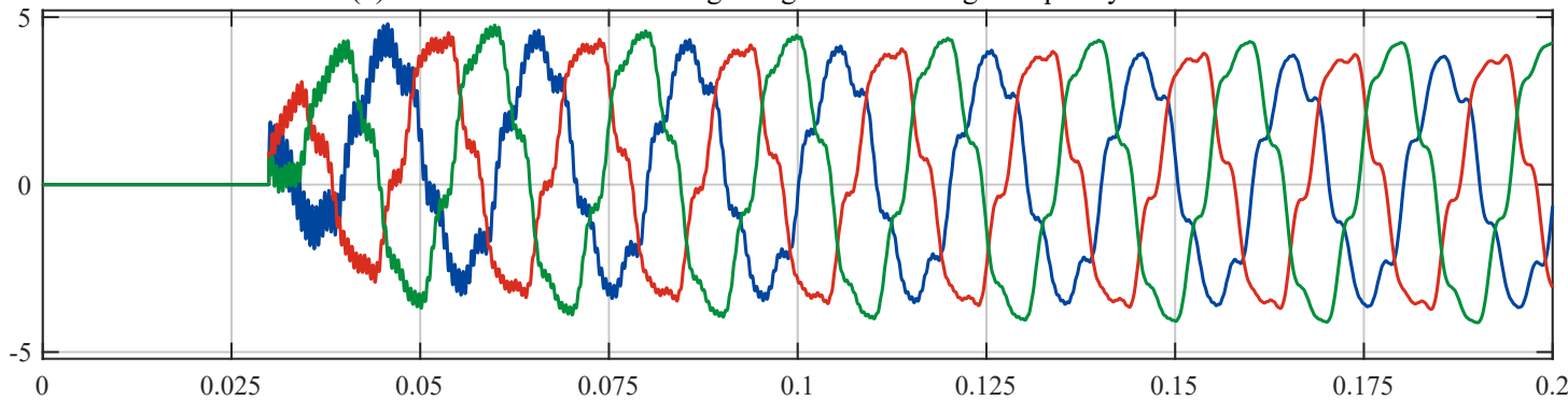
(d) Internal fault: sustained high magnitude with high-frequency transients
