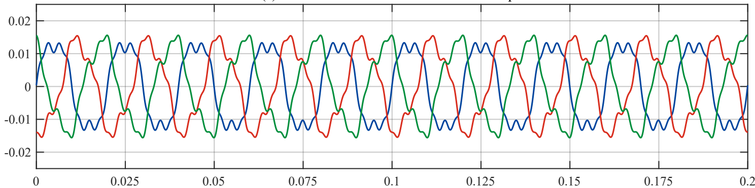
(b) External fault with CT saturation: transient spikes, THD \approx 34.7\%
