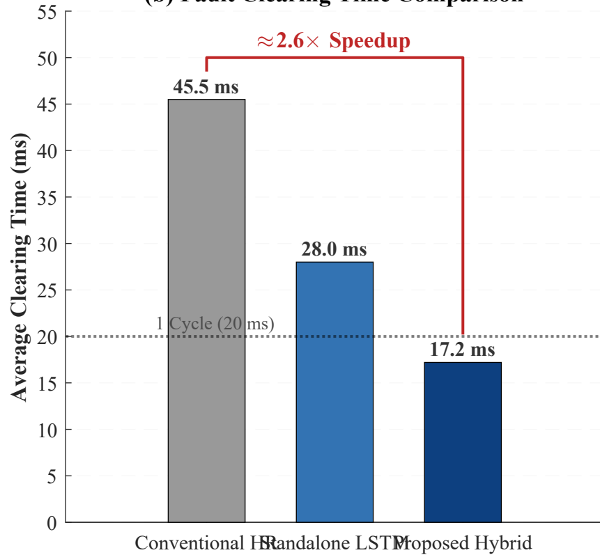
(b) Fault Clearing Time Comparison
