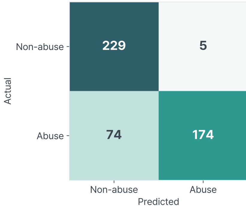
INT8 Quantized
