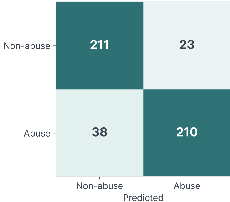
Original
