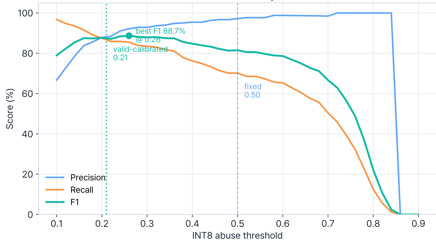
INT8 threshold sensitivity on test_set
