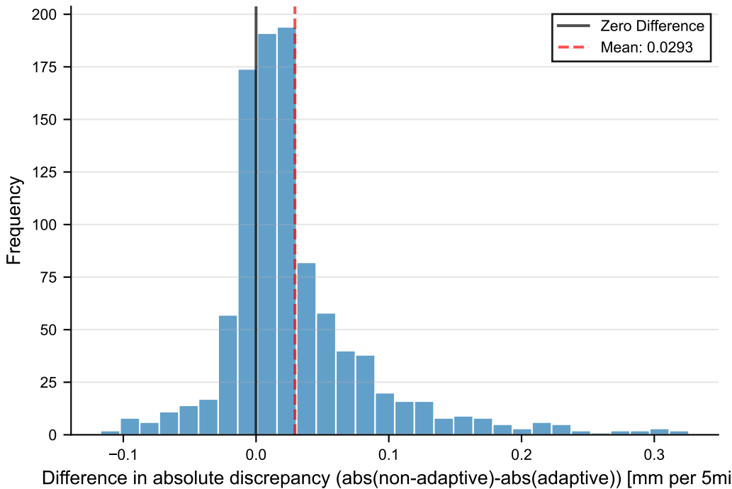
Distribution of Differences in Rainfall Depth Discrepancy
