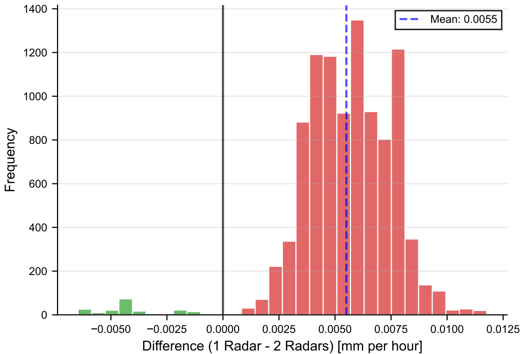
Distribution of Differences in Rainfall Depth
