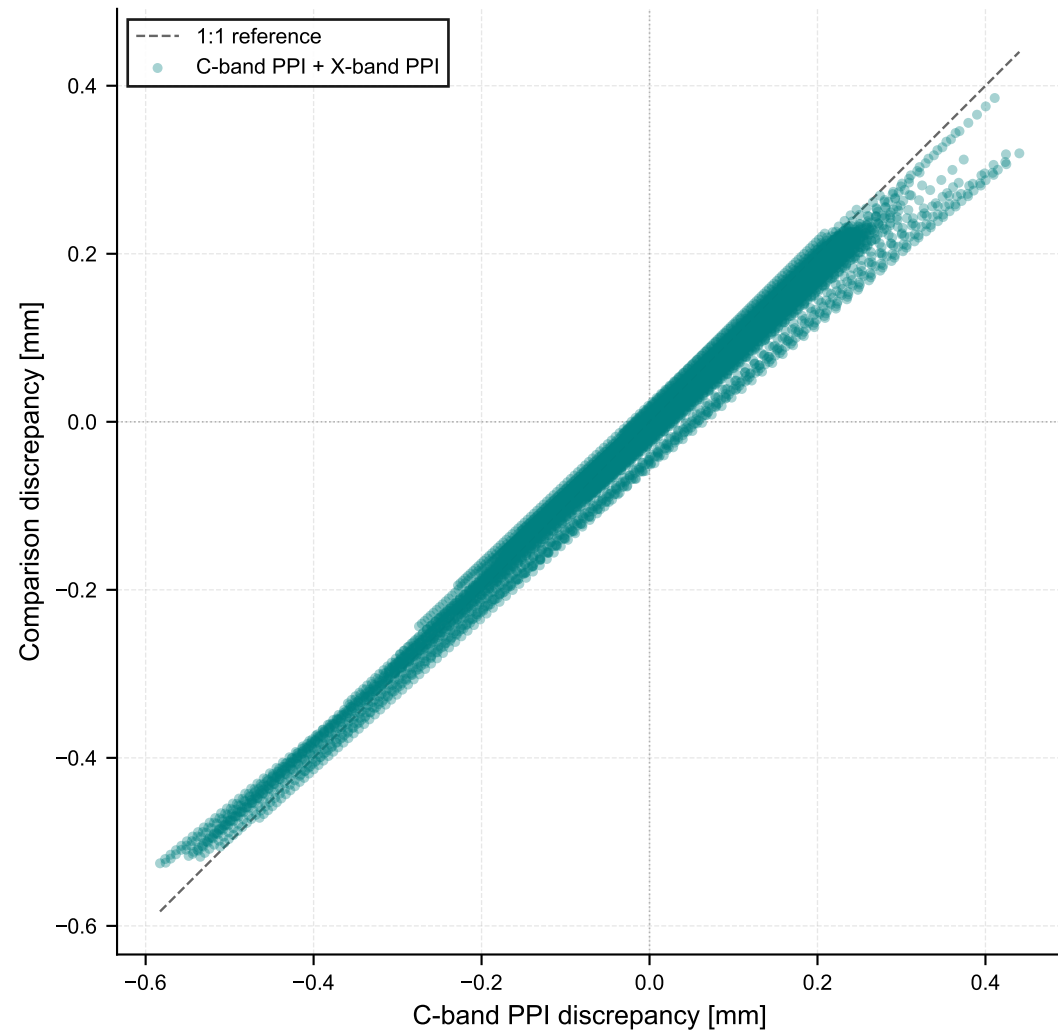
Combined vs C-band PPI
