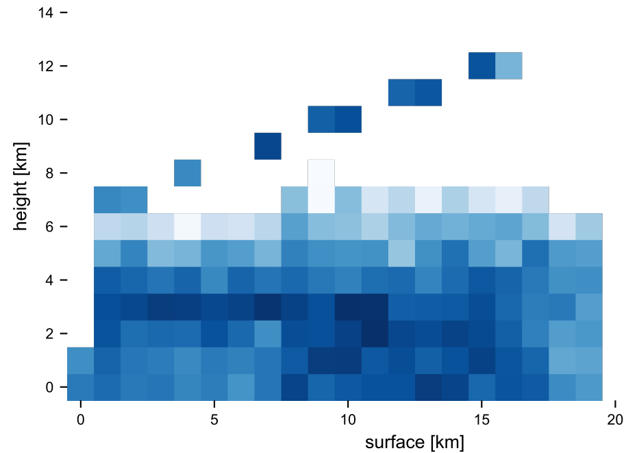
RHI Measured reflectivity (X-band)
