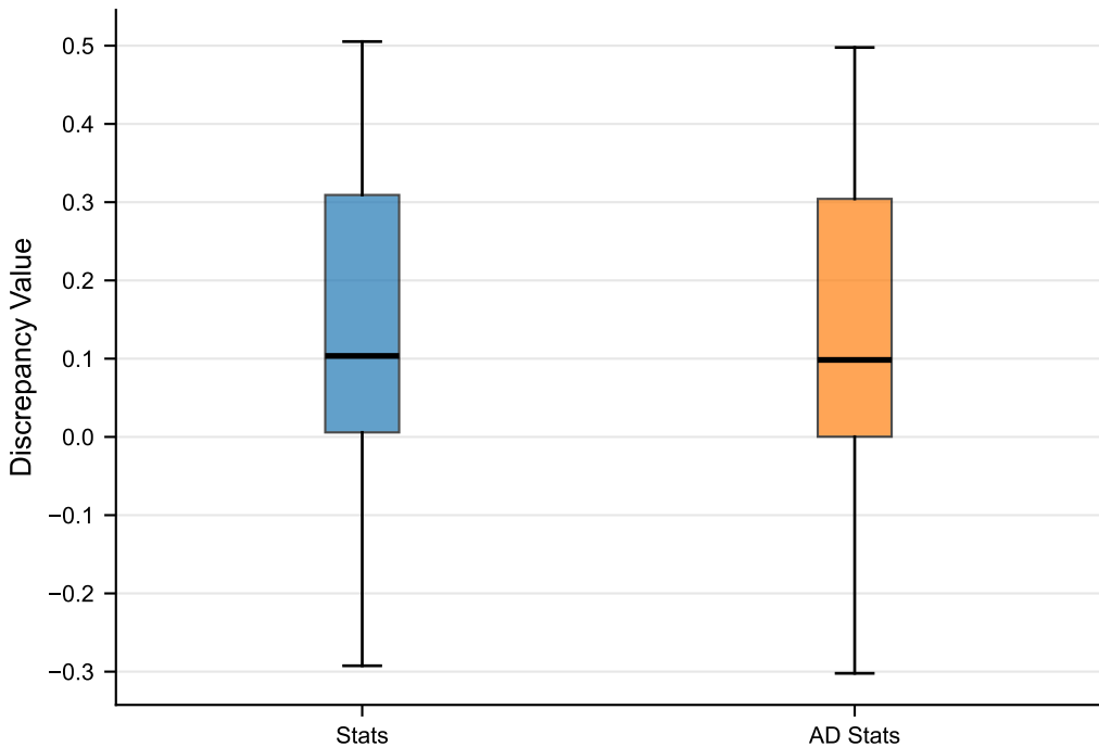
Boxplot Comparison: Stats vs AD Stats
