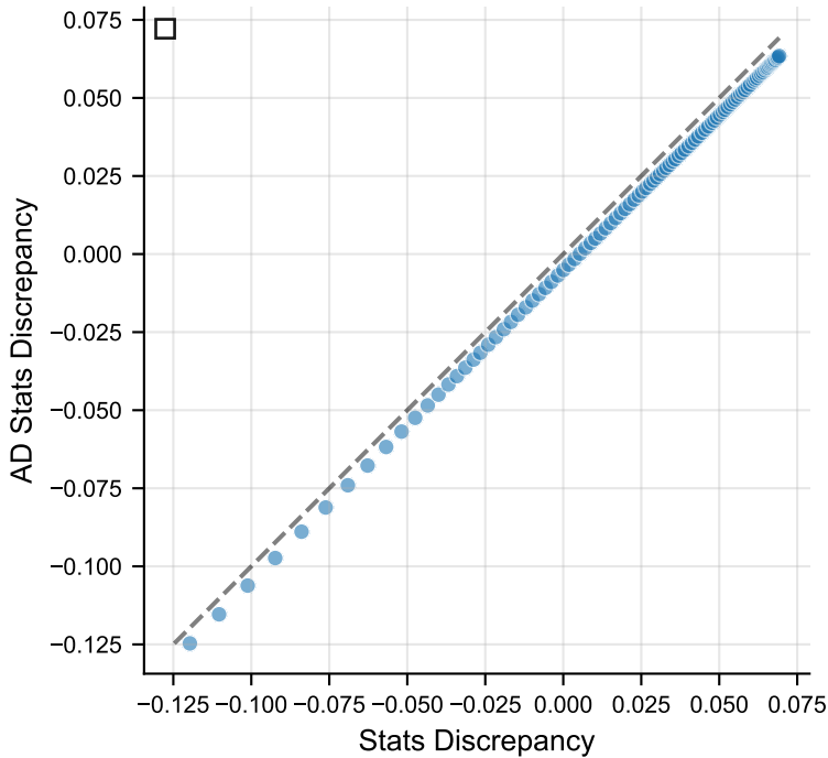
Scatter Plot: Stats vs AD Stats
