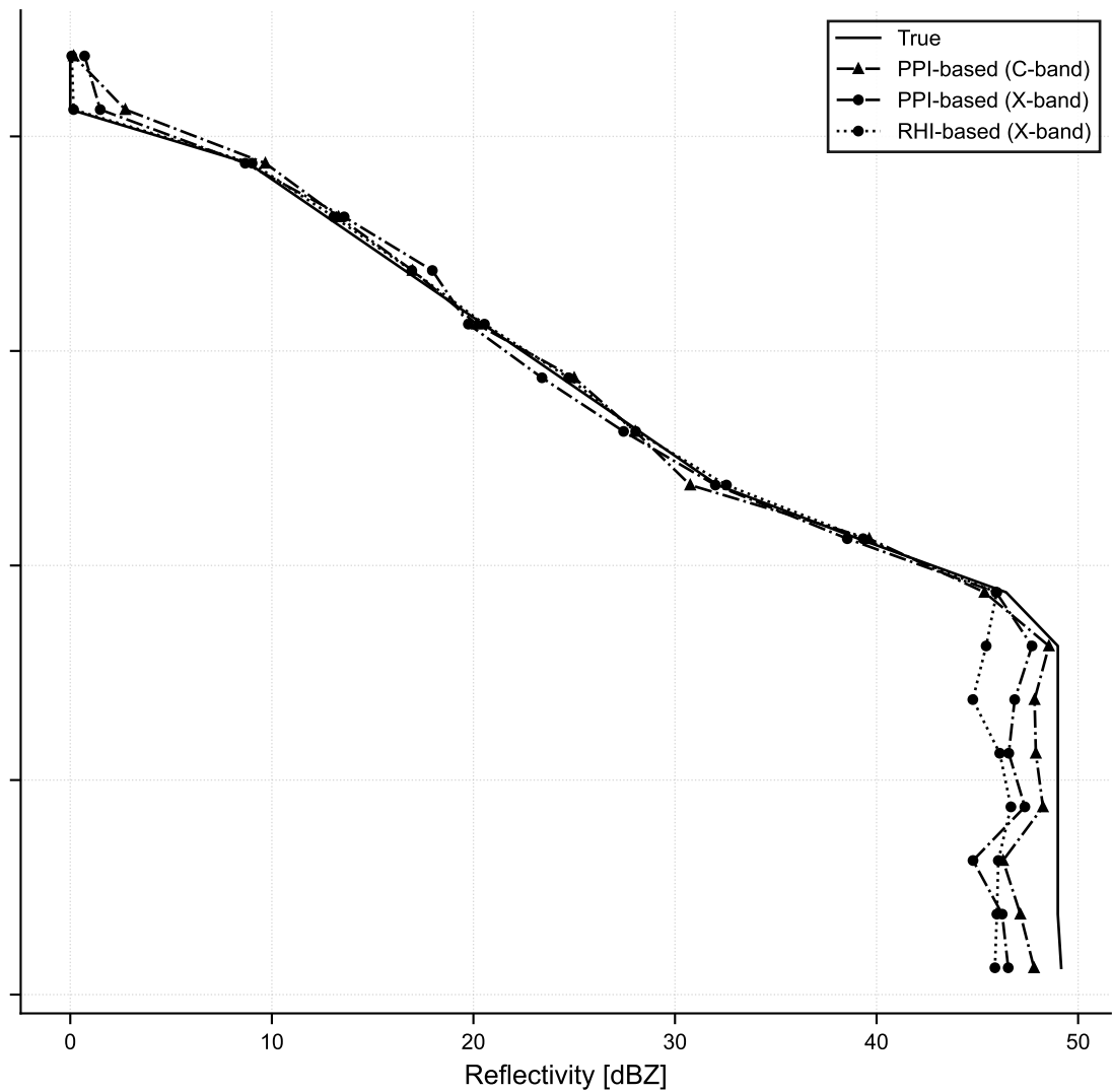
Convective VPR
