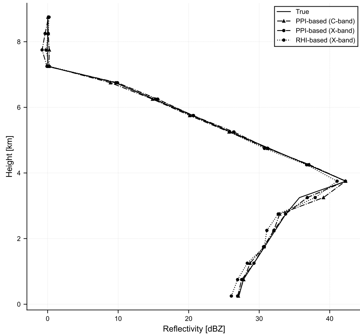
Stratiform VPR
