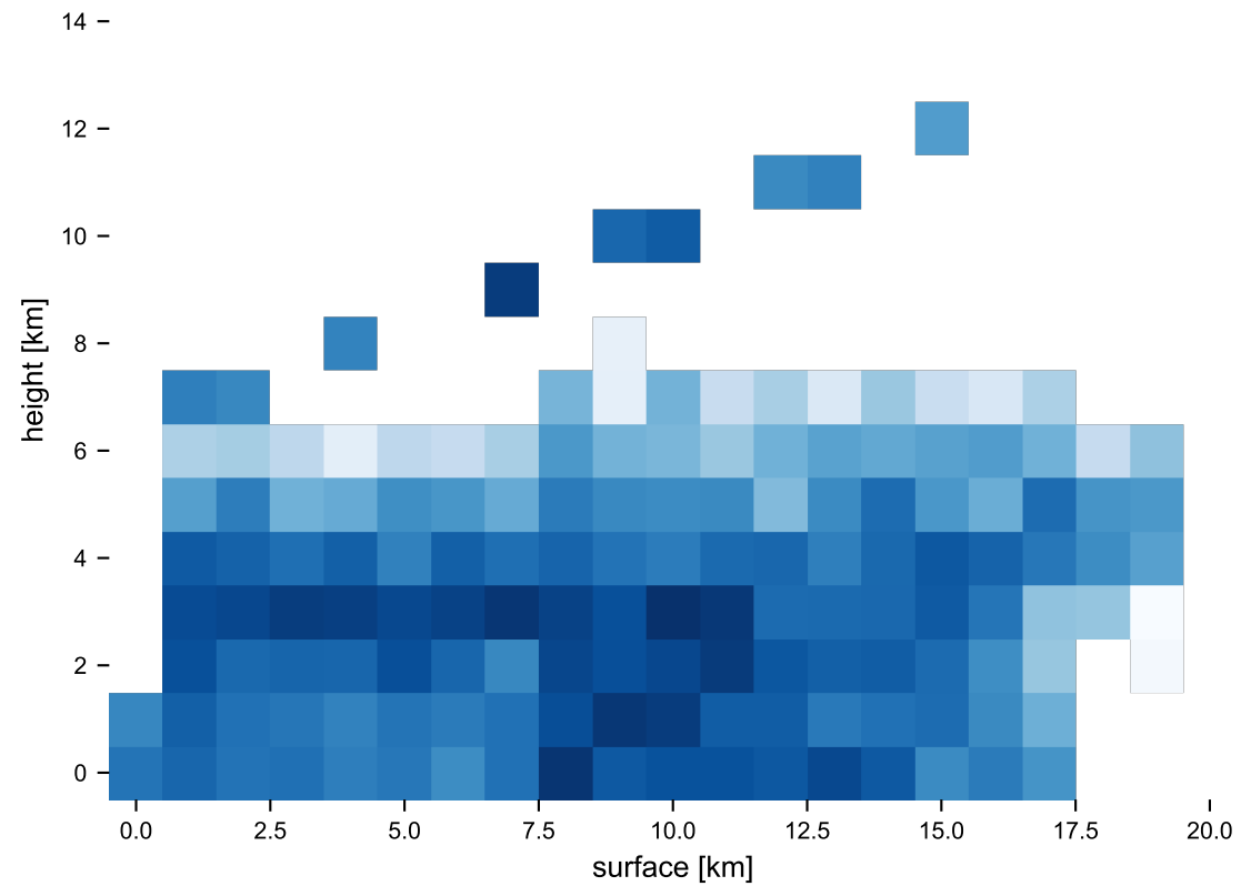
RHI True Reflectivity
