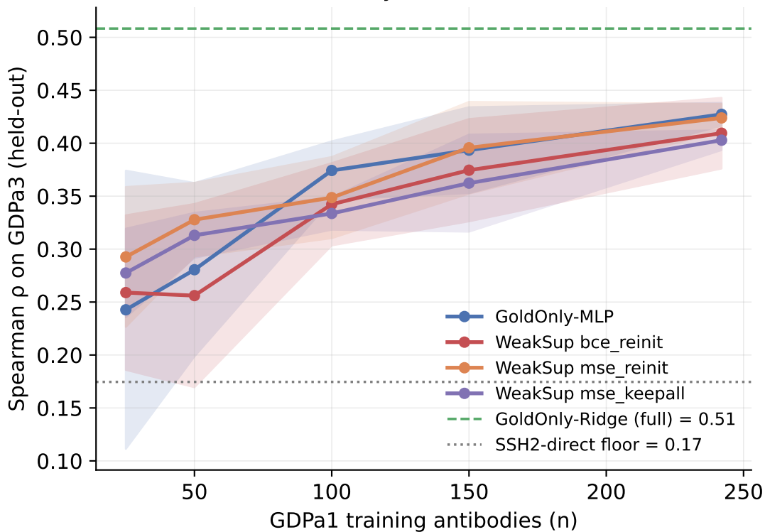
Data efficiency — esm2-650m / cls
