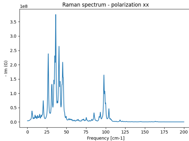
Figure 3.3: Raman spectrum with 200 iterations of the Lanczos algorithm along the x polarization for both incoming and outgoing radiation
