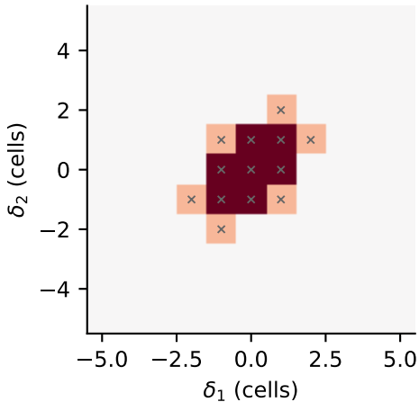
minimal-image target (violates ASR)
