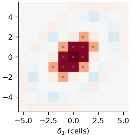
fitted, uniform class sums ( K = 3 , support 2L )
