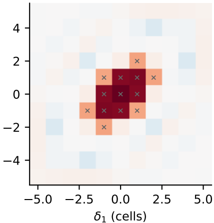
ASR-projected target (one-shot projection)
