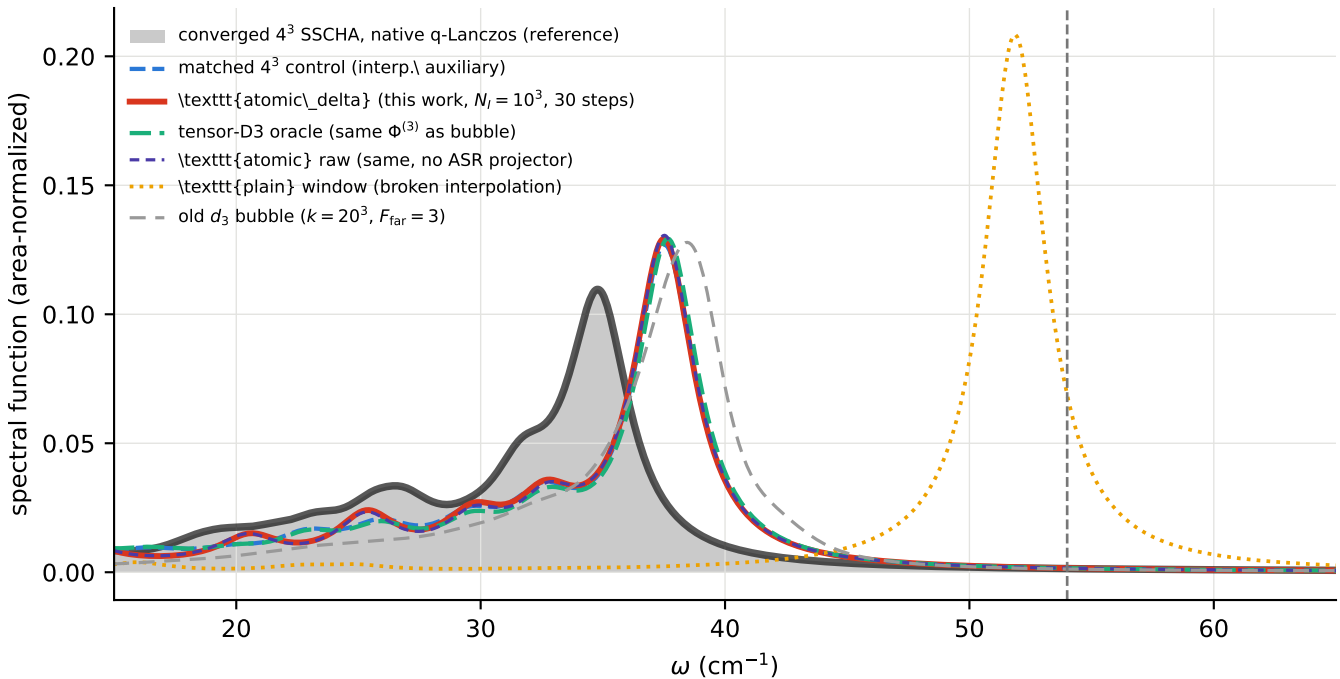
SnTe \Gamma TO spectral function --- 2^3 \rightarrow 4^3 interpolation, D_3 -only, T = 280 K, \sigma = 1.5 cm ^{-1}
