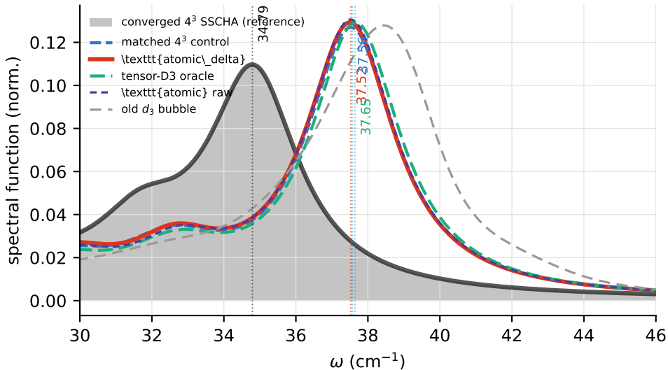
SnTe \Gamma TO --- zoom on the non-Lorentzian peak
