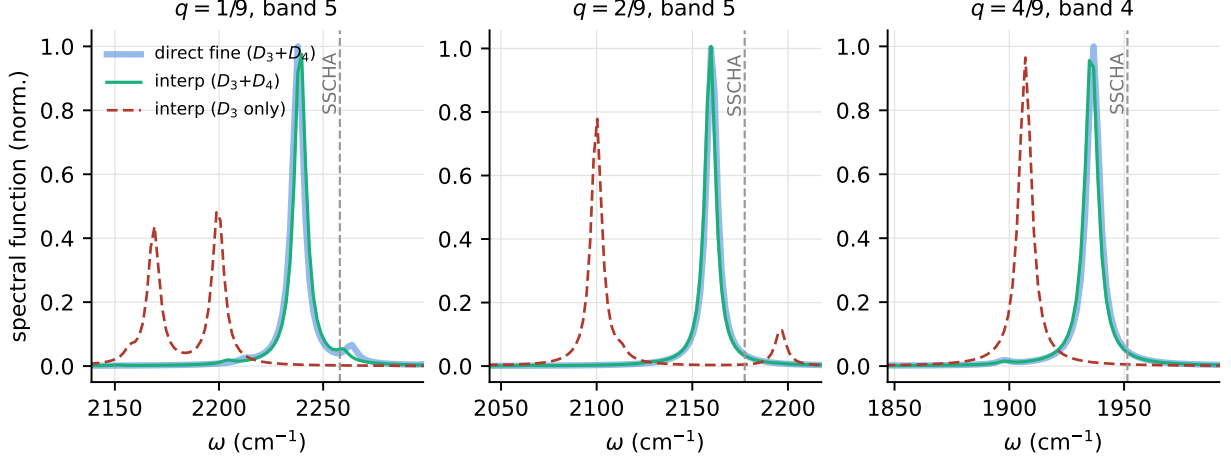
Figure 7: One-phonon spectral functions in a D_4 -dominated regime ( g_3 = 0.15 , g_4 = 2.0 ) at interpolated wavevectors of the (1, 1, 9) mesh. Blue: direct fine-mesh TDSCHA Lanczos ( D_3+D_4 ). Aqua: interpolated from the coarse (1, 1, 3) ensemble ( D_3+D_4 ) — it overlays the direct reference. Red dashed: the same interpolation with the fourth order dropped ( D_3 only), displaced by the quartic hardening of 30 \dots 56 \text{ cm}^{-1} . The SSCHA frequency is marked; curves normalized to the direct peak.
