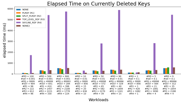
Figure 4: Elapsed time of testing on all of the deleted keys when \alpha = 0.9, T = 2, P = 32, E = 1024 . From left to right separated into 3 groups [(g1,g2,g3), (g4,g5,g6), (g7,g8,g9)], each of them has selectivity 0.001, 0.01, 0.1 respectively. While (g1,g4,g7) has 10% of total keys deleted and the middle three (g2,g5,g8) have 50%, whereas the tallest ones (g3,g6,g9) have 90% keys deleted.
