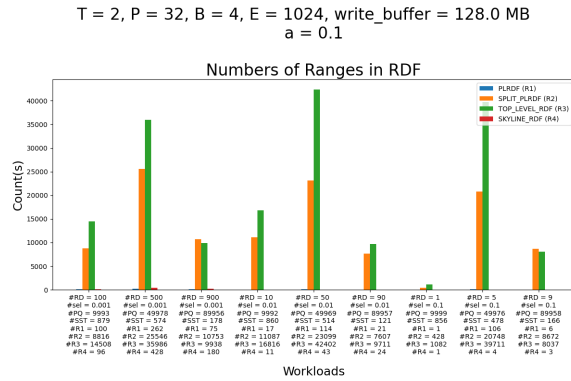
Figure 13: Number of ranges tested on all of the existing keys when \alpha = 0.1 , T = 2, P = 32, E = 1024. Over 9 workloads.
