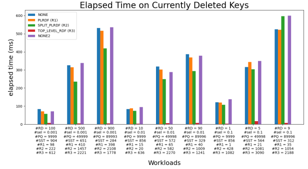
Figure 5: Elapsed time of testing on all of the deleted keys without Skyline when \alpha = 0.9, T = 2, P = 32, E = 1024 . From left to right separated into 3 groups [(g1,g2,g3), (g4,g5,g6), (g7,g8,g9)], each of them has selectivity 0.001, 0.01, 0.1 respectively. While (g1,g4,g7) has 10% of total keys deleted and the middle three (g2,g5,g8) have 50%, whereas the tallest ones (g3,g6,g9) have 90% keys deleted.
