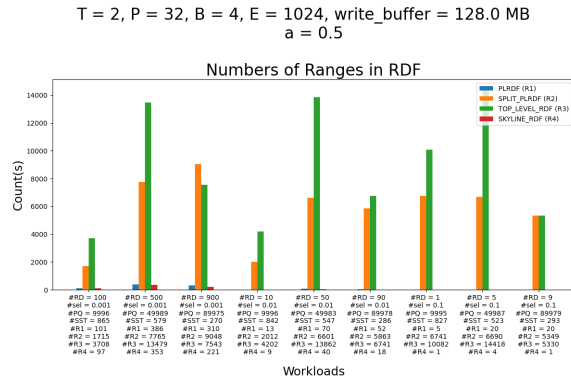
Figure 12: Number of ranges tested on all of the existing keys when \alpha = 0.5 , T = 2, P = 32, E = 1024. Over 9 workloads.
