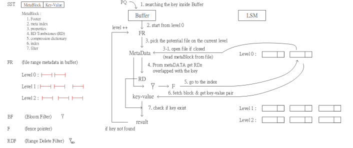
Figure 1: The flow of the PQ in RocksDB.
