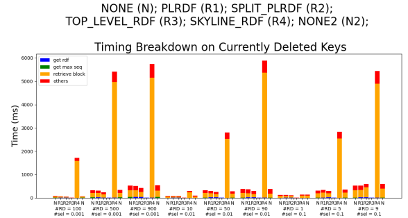
Figure 6: Timing breakdown of testing on all of the deleted keys when \alpha = 0.9, T = 2, P = 32, E = 1024 . Over 9 workloads.
