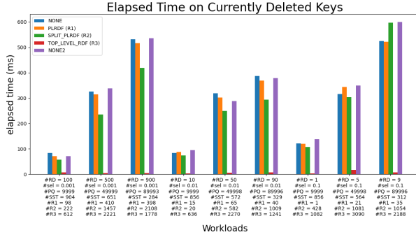
Figure 3: Elapsed time of testing on all of the deleted keys without Skyline when \alpha = 0.9 , T = 2, P = 32, E = 1024. From left to right separated into 3 groups [(g1,g2,g3), (g4,g5,g6), (g7,g8,g9)], each of them has selectivity 0.001, 0.01, 0.1 respectively. While (g1,g4,g7) has 10% of total keys deleted and the middle three (g2,g5,g8) have 50%, whereas the tallest ones (g3,g6,g9) have 90% keys deleted.
