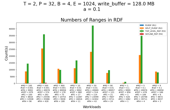
Figure 11: Number of ranges tested on all of the existing keys when \alpha = 0.1 , T = 2, P = 32, E = 1024. Over 9 workloads.
