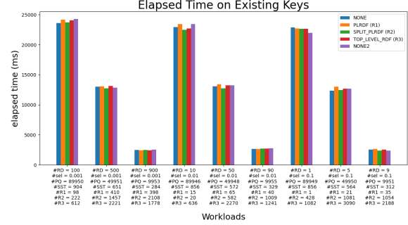
Figure 5: Elapsed time of testing on all of the existing keys when \alpha = 0.9 , T = 2, P = 32, E = 1024. Over 9 workloads.
