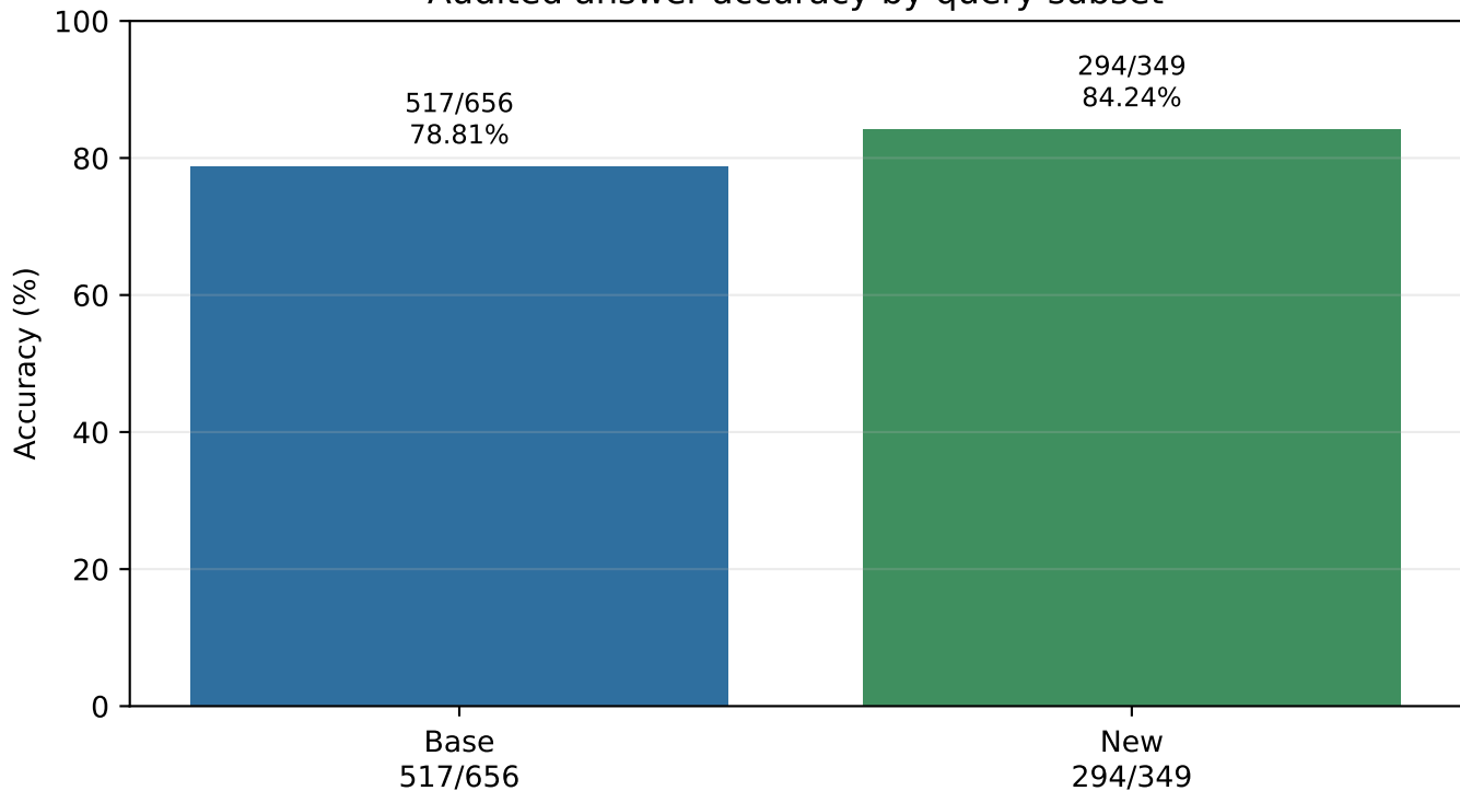
Audited answer accuracy by query subset
