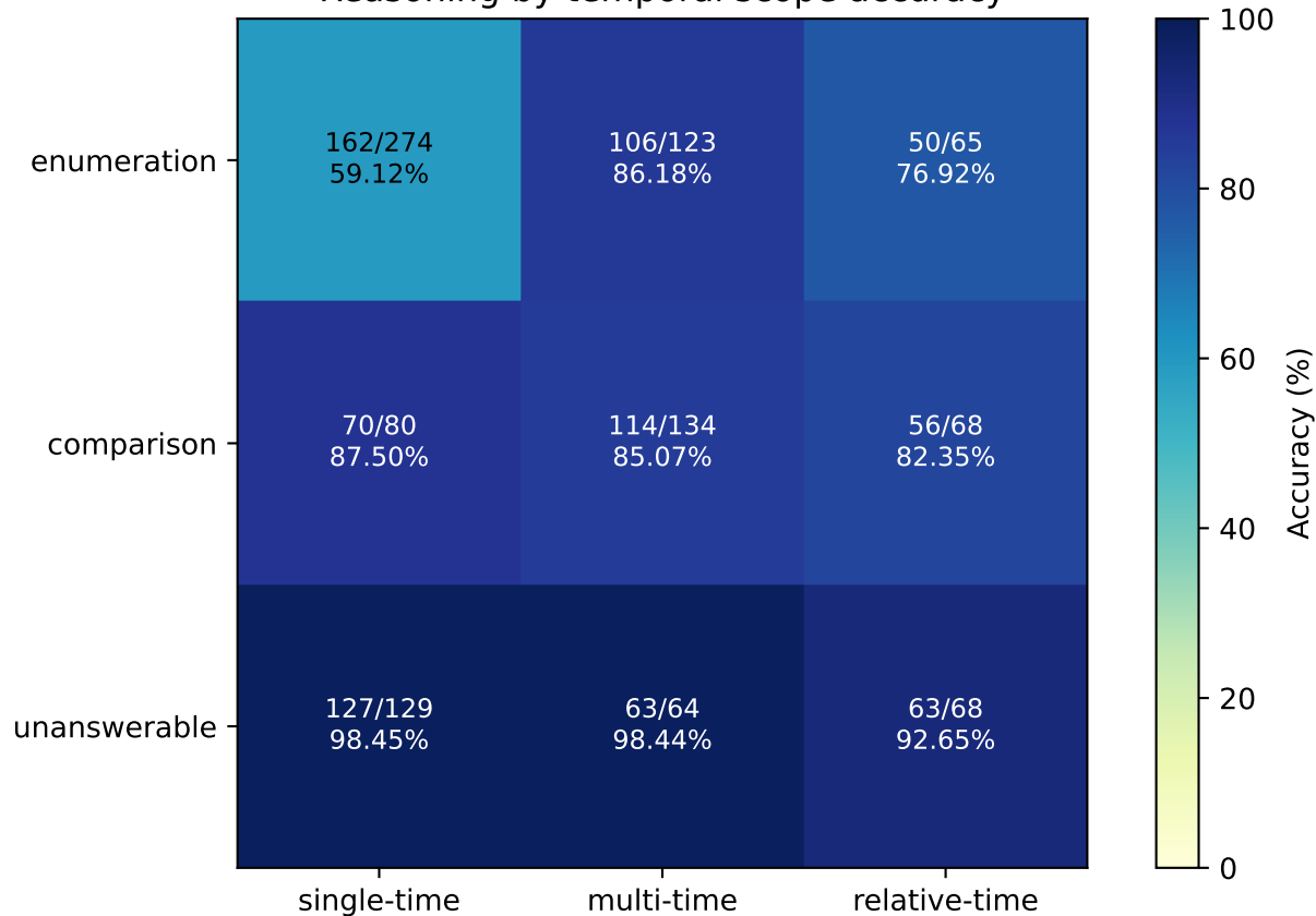
Reasoning by temporal scope accuracy
