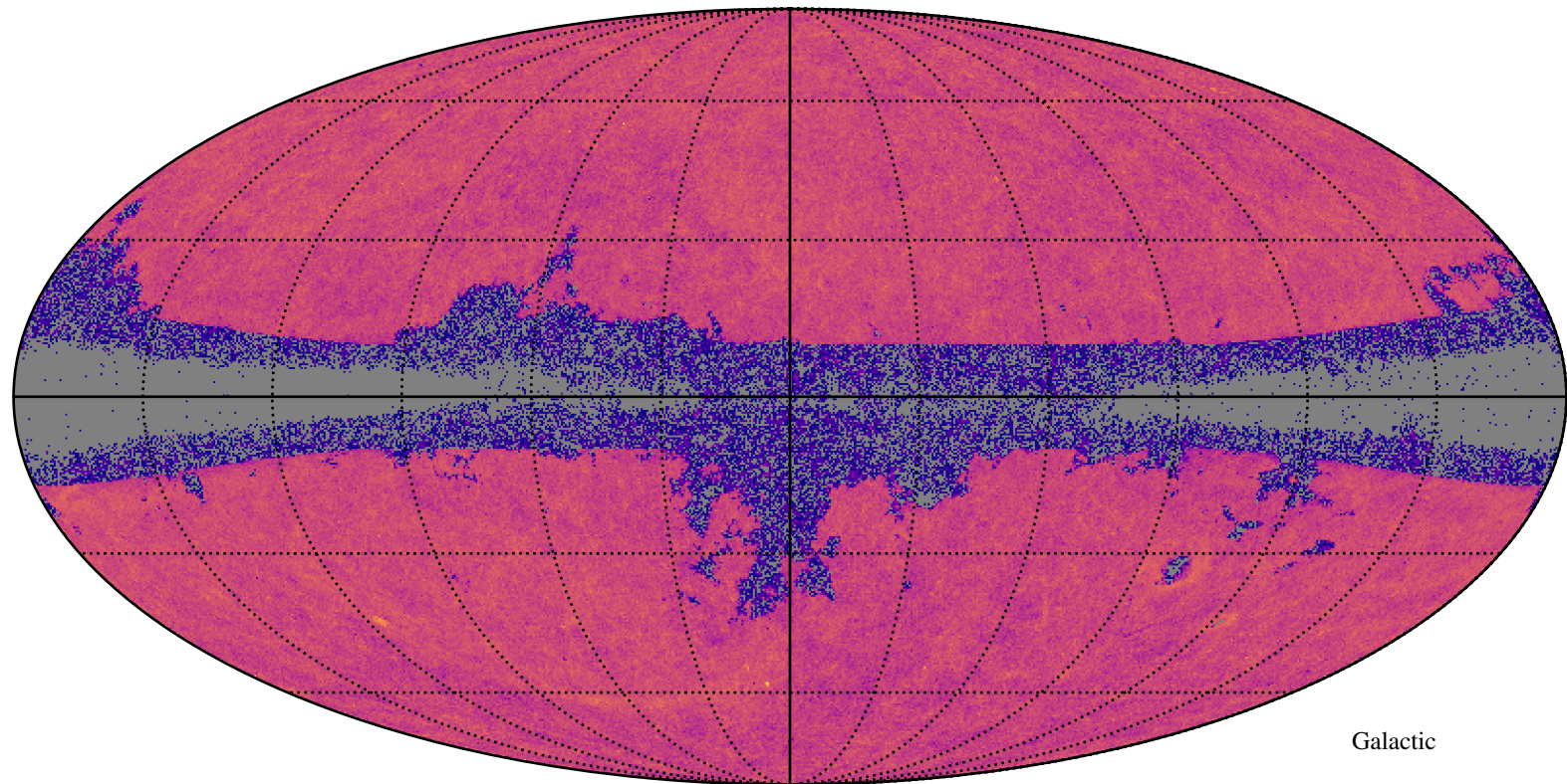
GLADE+ Galaxy Distribution (Galactic Coordinates)
