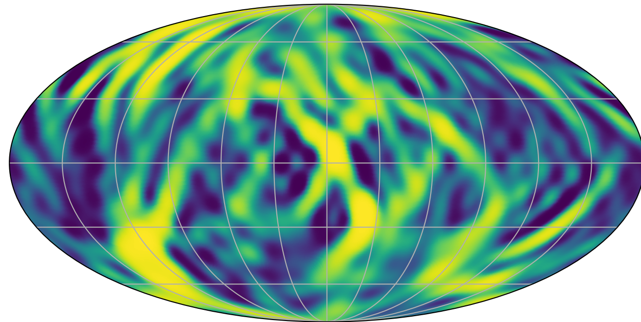
GW Localization Skymap (GWTC-4; \ell \leq 26 )
