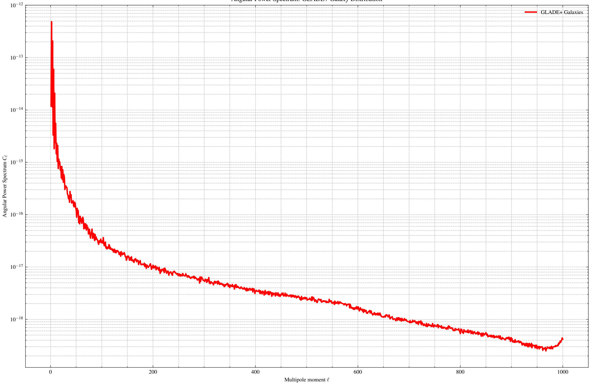
Angular Power Spectrum: GLADE+ Galaxy Distribution
