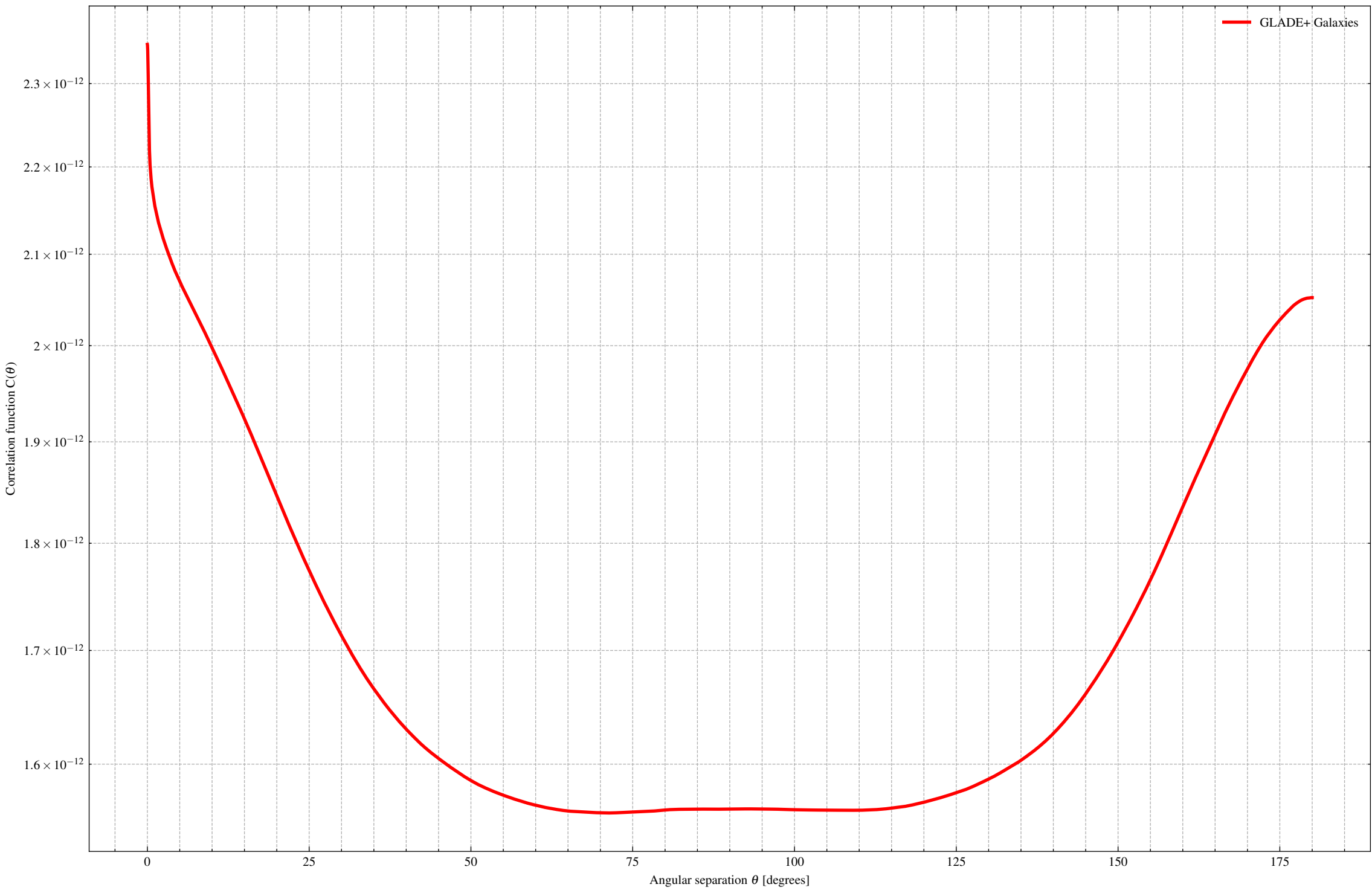
Angular Correlation Function: GLADE+ Galaxy Distribution
