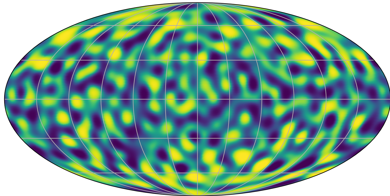
GRB Event Density Skymap ( \ell \leq 26 )
