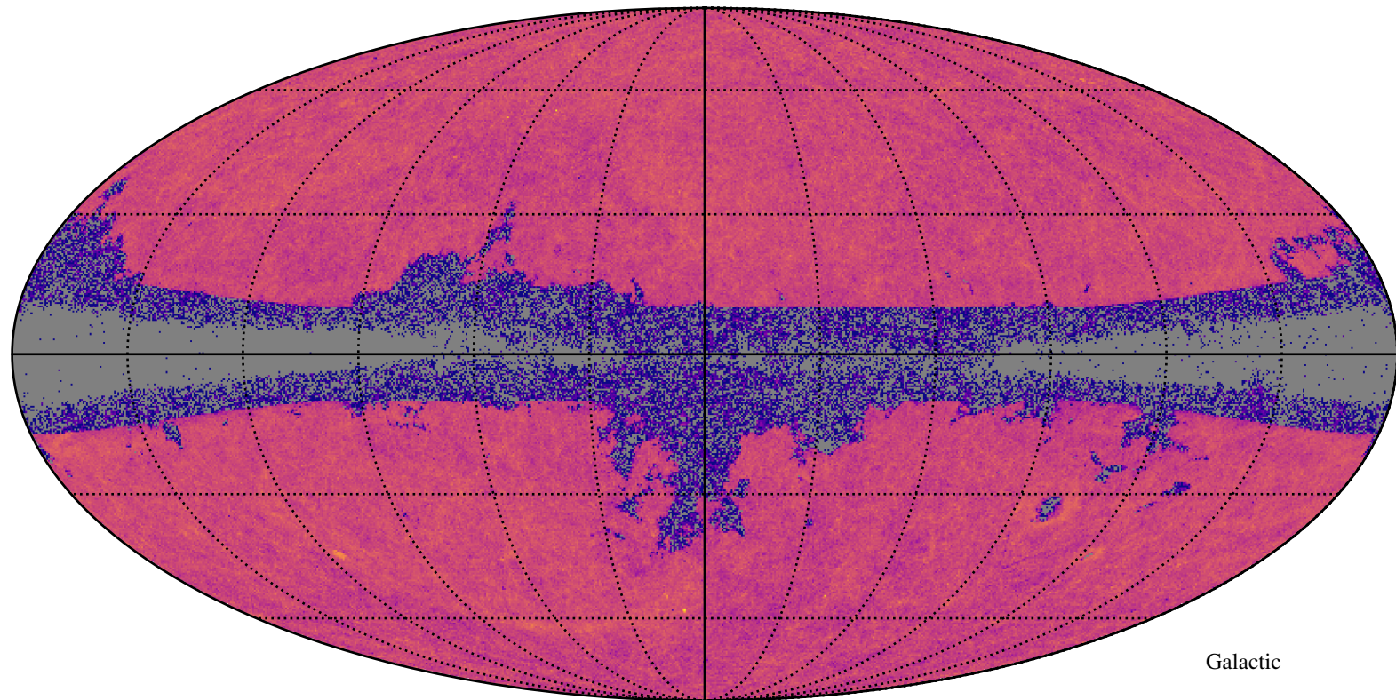
GLADE+ Galaxy Distribution
