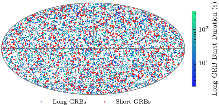
GRB Skymap
