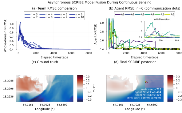
Fig. 3. Asynchronous fusion during continuous sensing. Circles mark peer encounters in the selected six-agent mission; the bottom row compares its final model with the ROMS ground truth.
