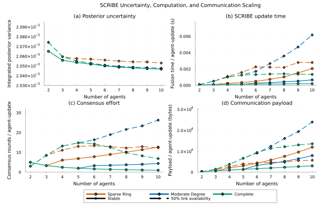
Fig. 4. Uncertainty, computation, and communication scaling across team sizes, network densities, and link conditions. Dashed curves denote 50% link availability.
