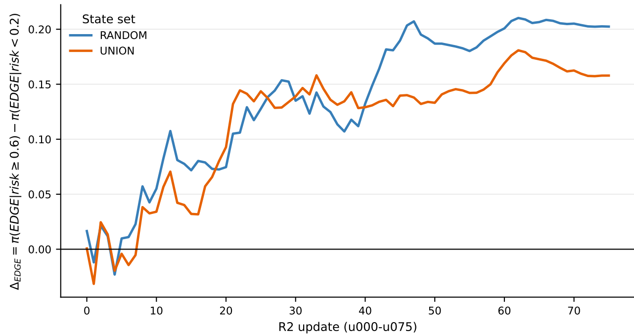
Figure 8. Sprint 7 R2 \Delta\_EDGE trajectory on frozen state sets
