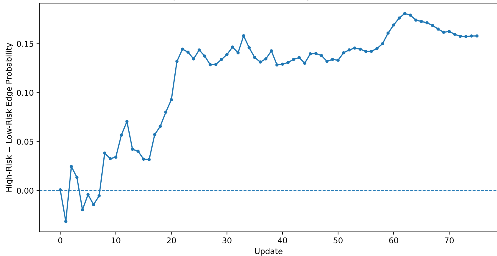
Sprint 7: Risk-Conditioned Edge Preference
