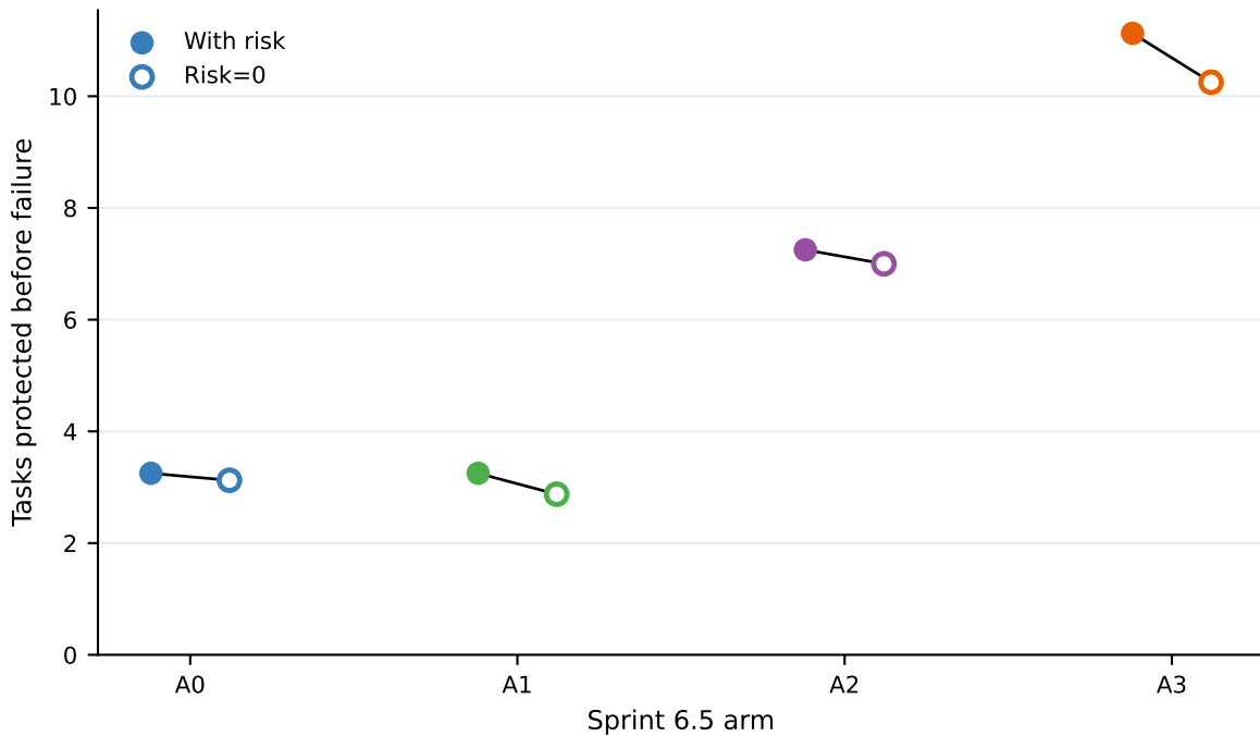
Figure 7. Zero-risk ablation: physical protection (8 held-out episodes/arm)
