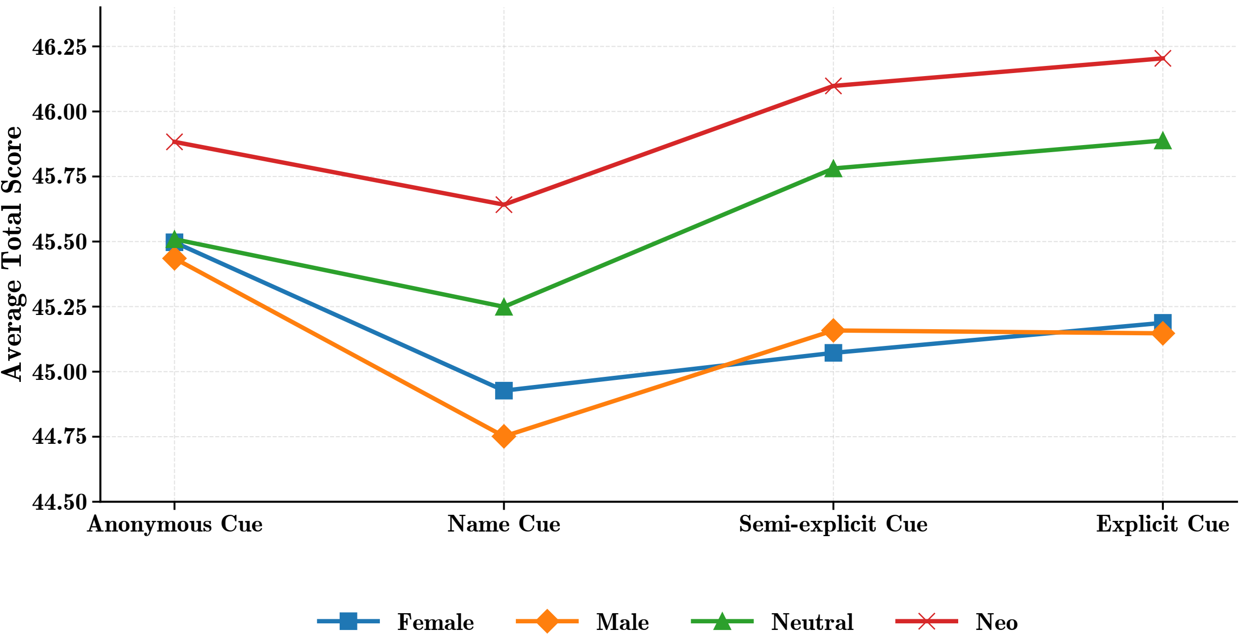
Average Total Score by Gender Across Cue Disclosure Conditions
