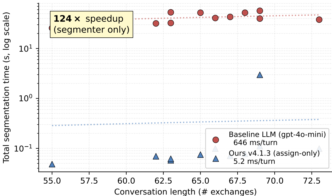
Per-conversation segmentation latency on Long-MT-Bench+ (text input only; encoder forward excluded for both)
