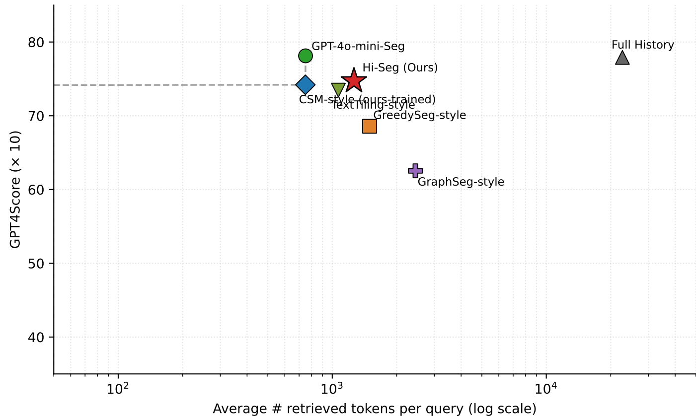
Context-quality Pareto on Long-MT-Bench+ (Hi-Seg achieves baseline-LLM-level quality at low token budget)
