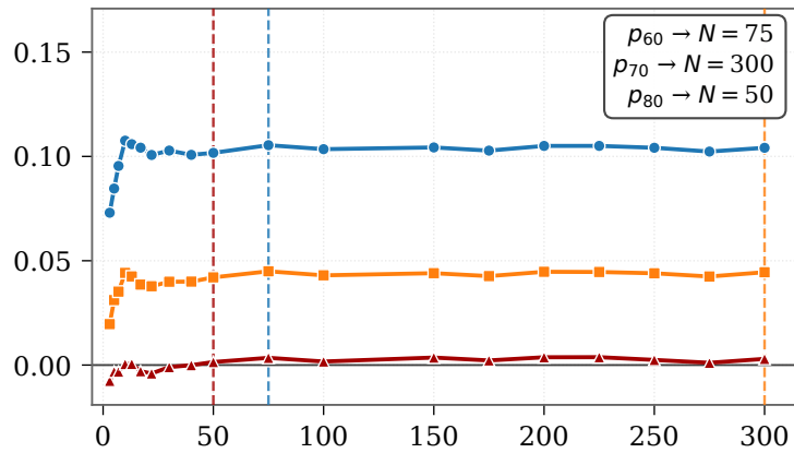
Dialseg711
