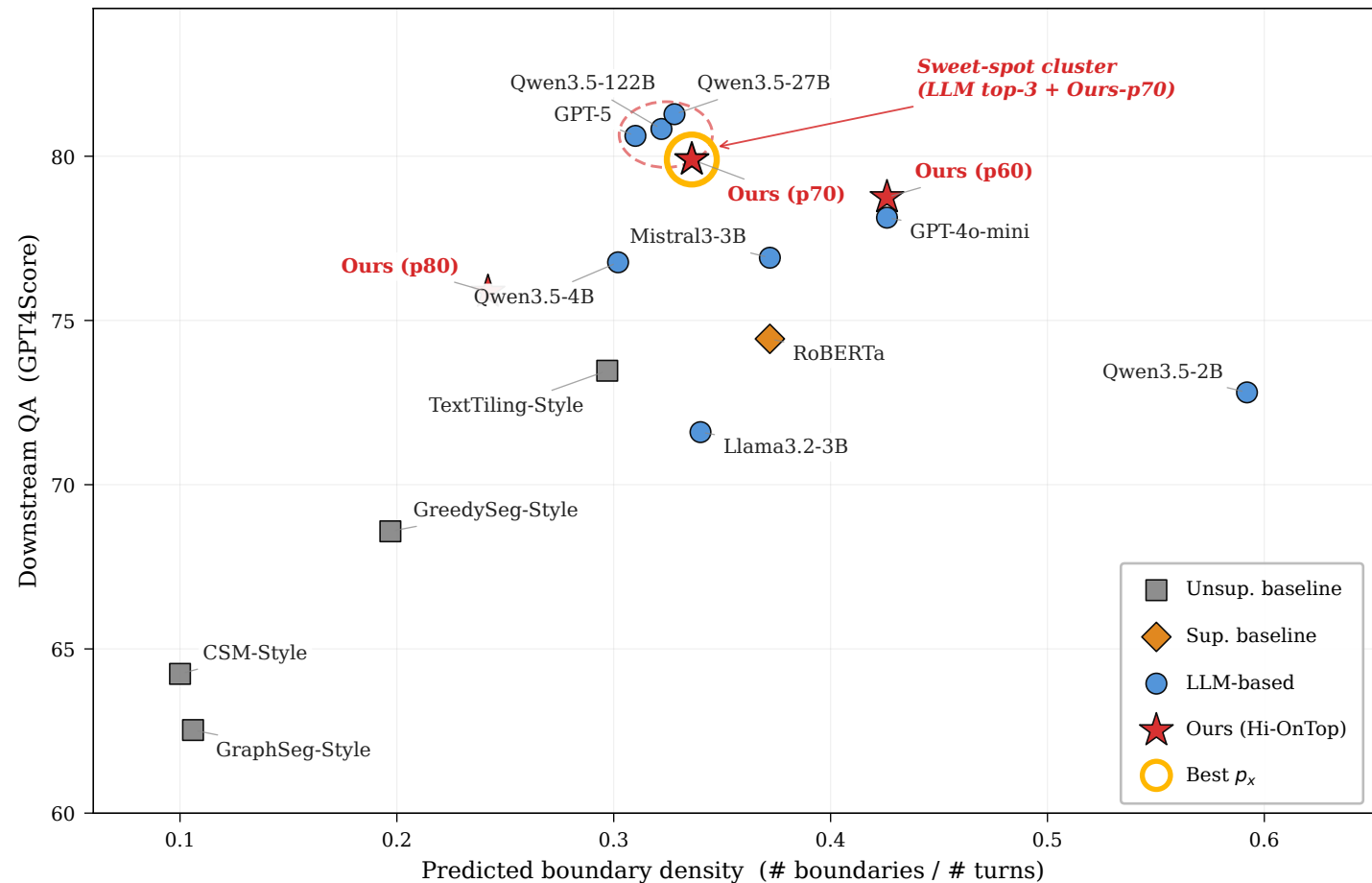
Boundary density vs downstream QA on Long-MT-Bench+
