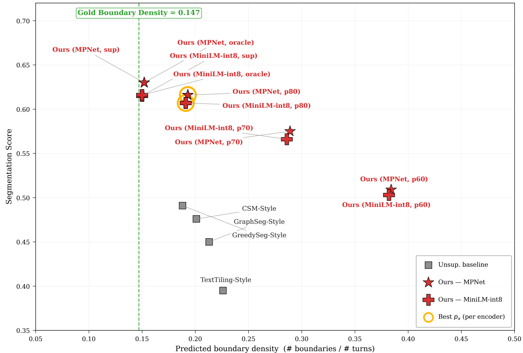
Boundary density vs Segmentation Score — Dialseg711
