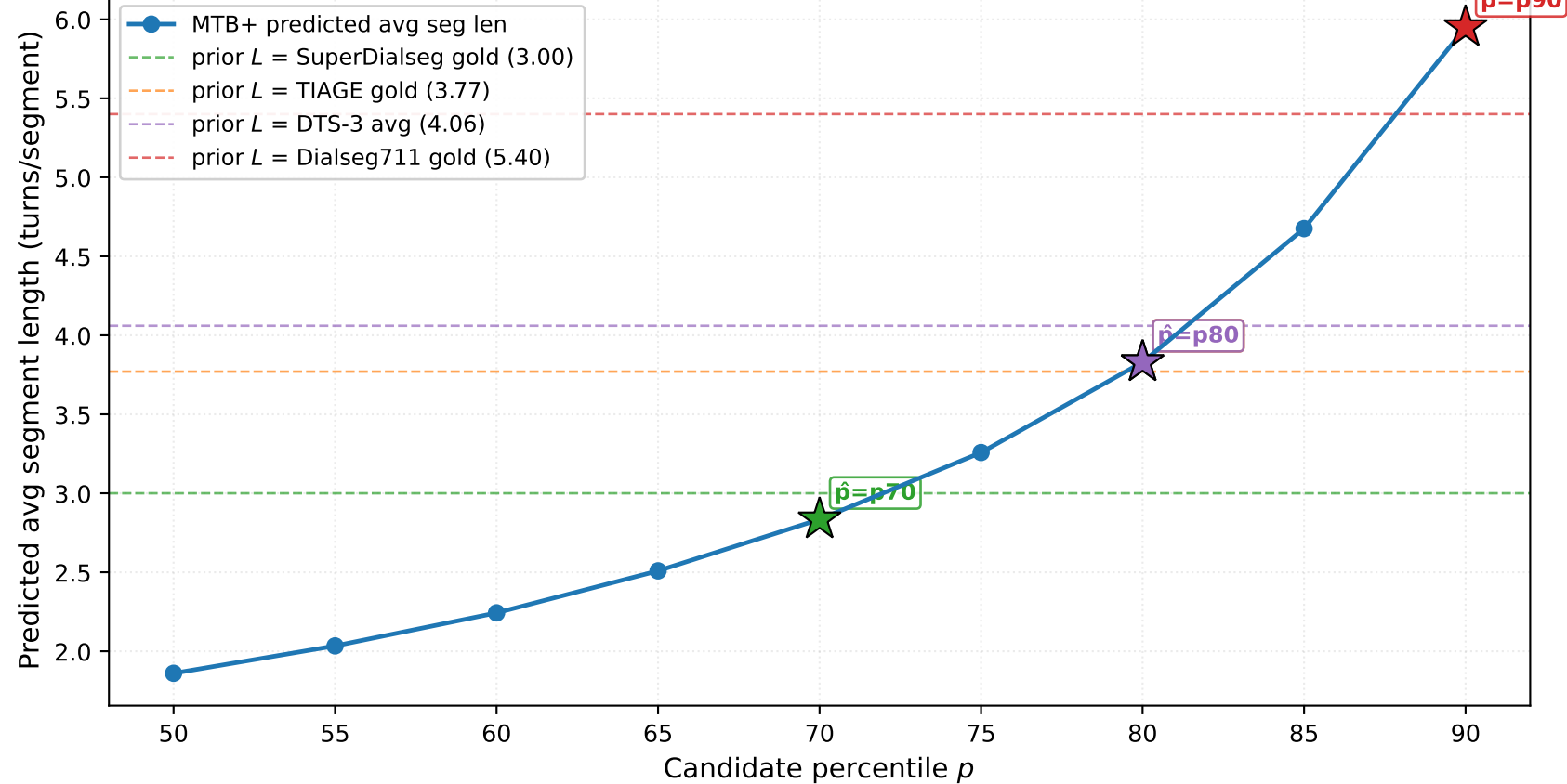
Label-free best- p via segment-length prior matching (MTB+, MiniLM-int8 encoder, no deployment labels used)
