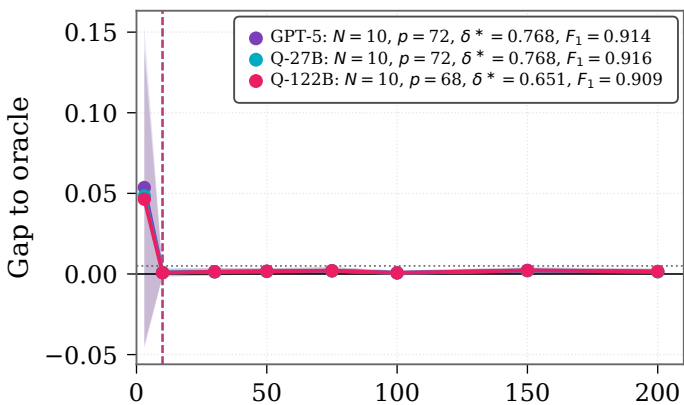
MiniLM-int8
