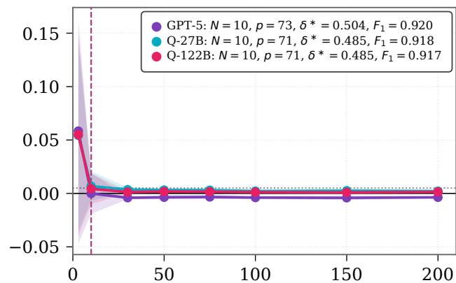
MPNet
