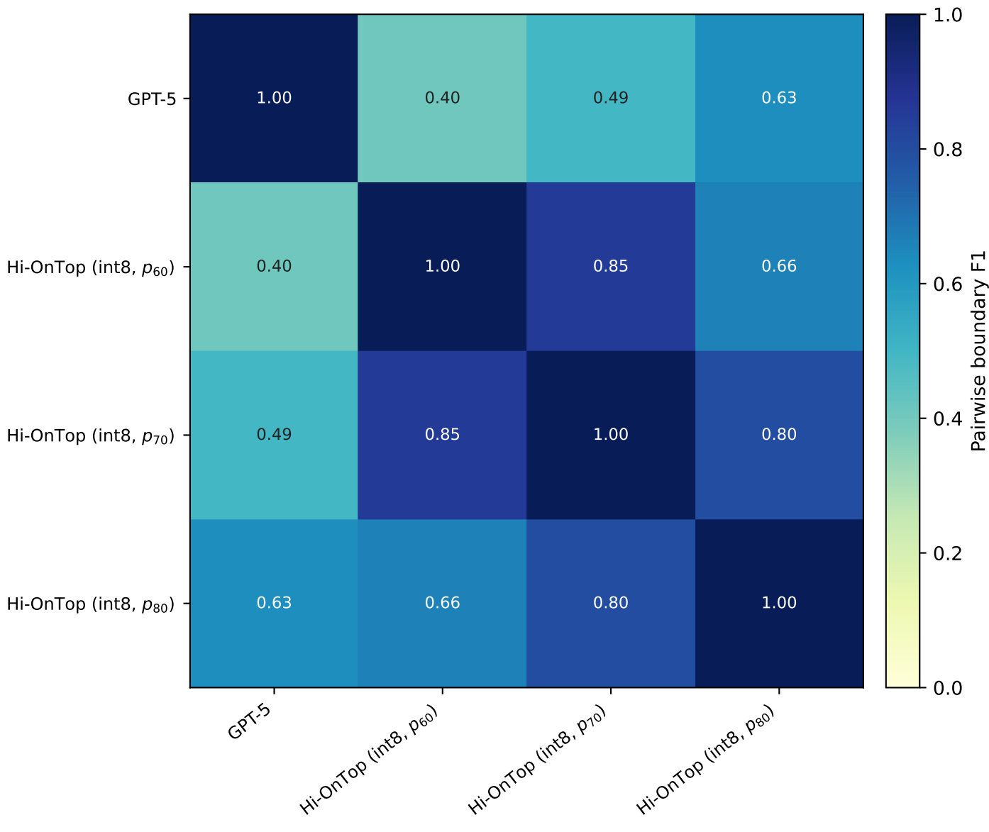
Pairwise boundary F1 on LongMemEval-S (360 instances, 4 methods)
