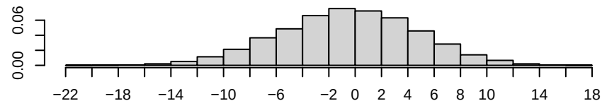
Density of b1degree1
