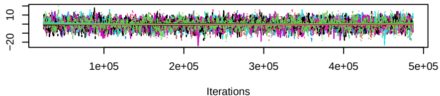
Trace of b1degree1
