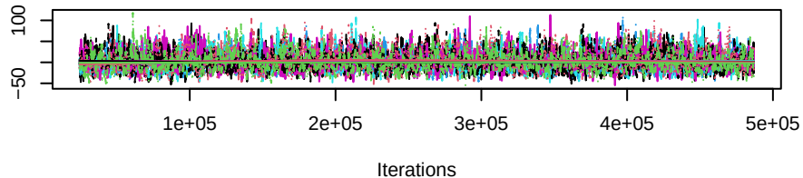
Trace of cycle4
