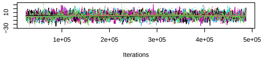
Trace of edges
