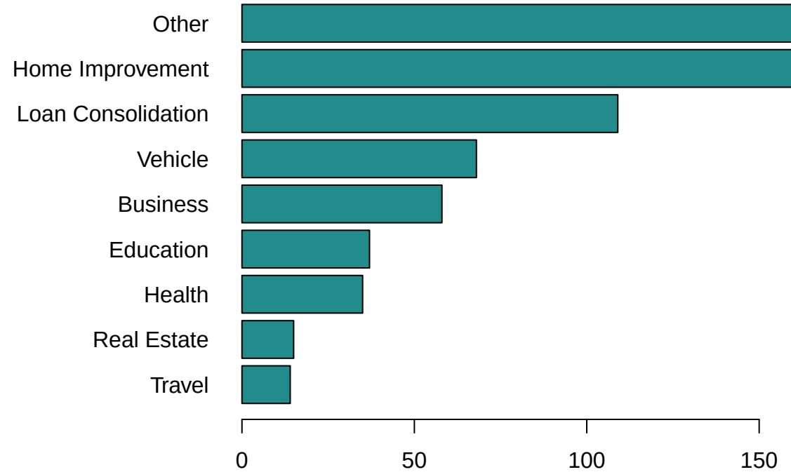
Reduced Sample
