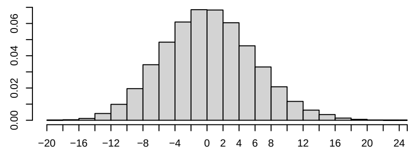
Density of b1factor.b1_gender.male
