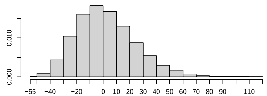
Density of cycle4
