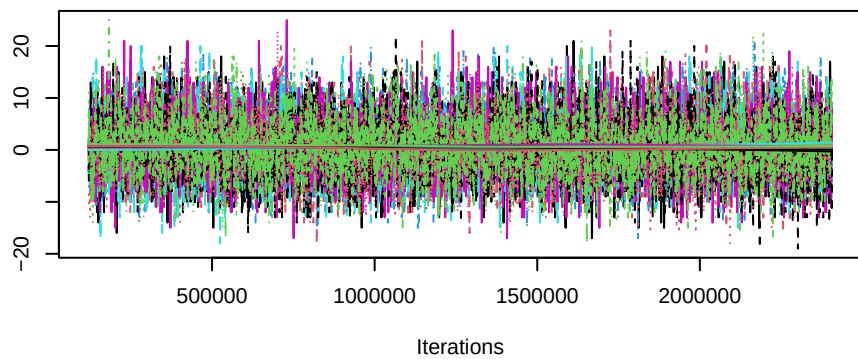
Trace of b1factor.b1_gender.male
