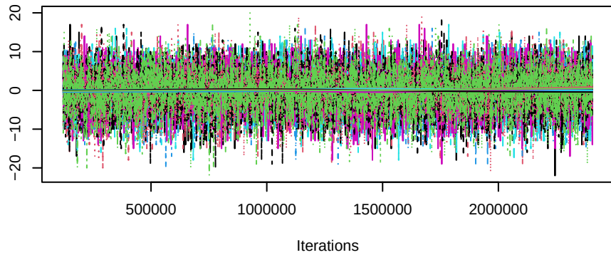
Trace of b1degree1
