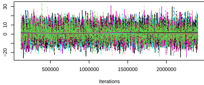
Trace of edges
