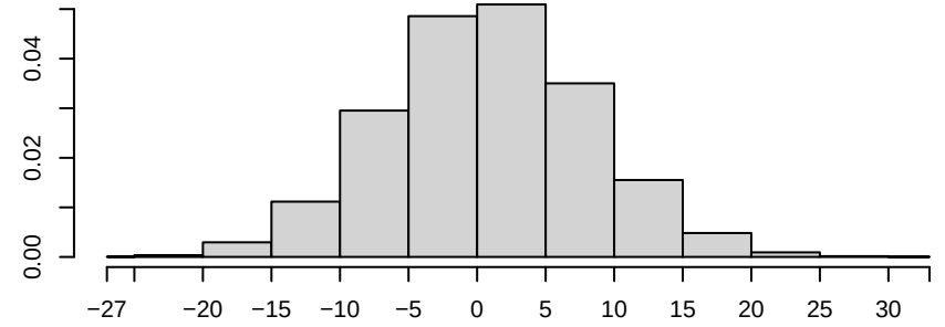
Density of edges
