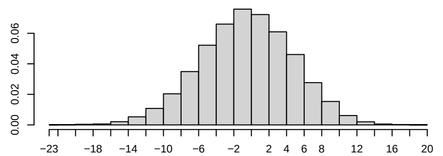
Density of b1degree1
