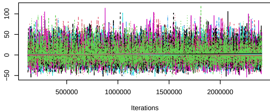
Trace of cycle4
